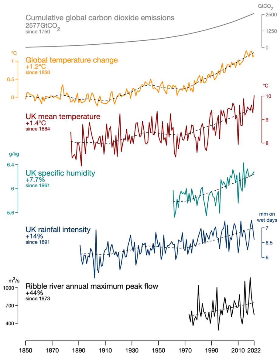
65 Figure 1: An observation-based causal chain from global carbon dioxide emissions to peak flow in the Ribble river. Cumulative anthropogenic global carbon dioxide emissions (grey; Friedlingstein et al. 2023) are causing global temperatures to increase (orange, with 41-year loess smoothed version in dashed black; Morice et al. 2021). Global warming is experienced locally as warmer UK temperatures (red), increased specific humidity (green), with corresponding increases in rainfall intensity (blue); all based on data from Hollis et al. (2019). Annual maximum peak flow on the Ribble river has increased in the last 50 70 years (black; NRFA 2023). Black dashed lines show regressions onto the smoothed global temperature timeseries.
