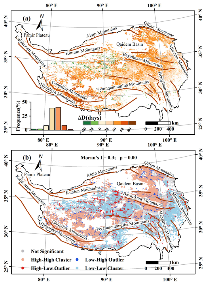
Figure 3: (a) Spatial, frequency distribution histogram and (b) local and global Moran's I value of average \Delta D on the Tibetan Plateau over 2001–2018.
