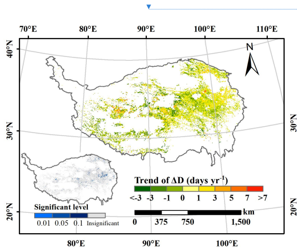
Figure 4: Interannual variation trend and significant levels of \Delta D on the Tibetan Plateau from 2001–2018.
