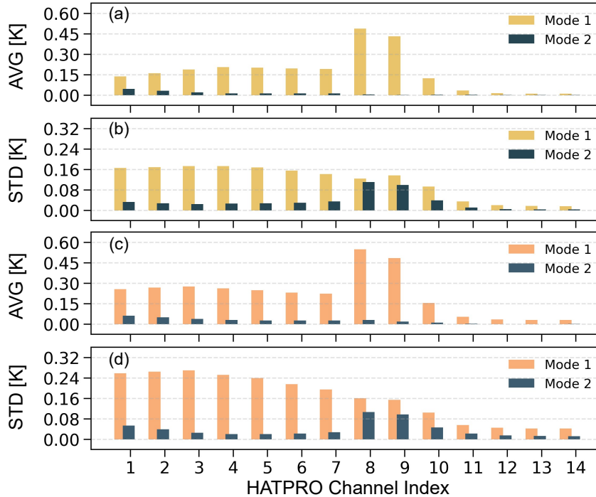
Figure 2. (a) and (b): AVGs and STDs of simulated BTs at 7 observed zenith angles in HATPRO channels. RT simulations for both interpolation mode 1 and 2 performed under the 54L ECMWF 83-profile dataset. MonoRTM serves as a benchmark to provide reference values for comparison. (c) and (d): Same as (a) and (b), but with RT simulations performed under the 54L UMBC 48-profile dataset.
