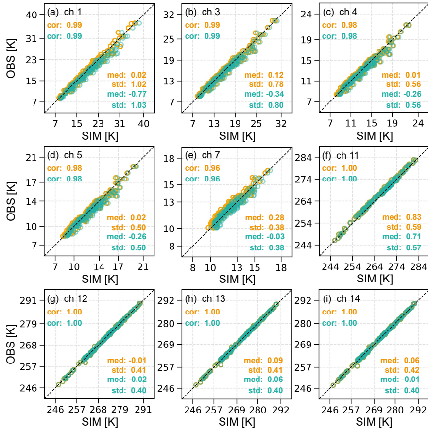
Figure 5. Scatter of simulated vs. observed BTs for 9 out of the 14 channels of Airda-HTG4 at Karamay from November 1, 2023 to April 30, 2024. RT simulations are performed using radiosonde data. Orange represents results of RTTOV-gb; Green represents results of ARMS-gb. After collocation and cloud detection, a total of 163 samples are analyzed in this case. The panel reports the correlation coefficients (cor), as well as the median values (med) and standard deviations (std) of OMB.
