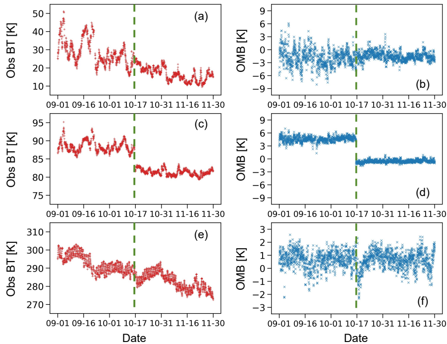
Figure 8. (a) and (b): Observations for channel 1 from Airda-HTG4 at Minfeng during September 1, 2023 to November 30, 2023 along with the corresponding OMB series of ARMS-gb. (c) and (d): Same as (a) and (b) but show situations of channel 8. (e) and (f): Same as (a) and (b) but show situations of channel 14. The green dashed line indicates the calibration time.
