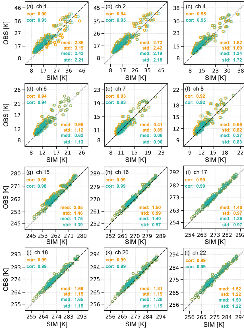
Figure 7. Same as Fig. 5, but shows results for 12 out of the 22 channels of YKW3 at Tanggu from November 1, 2023 to April 30, 2024. After collocation and cloud detection, a total of 148 samples are analyzed in this case.
