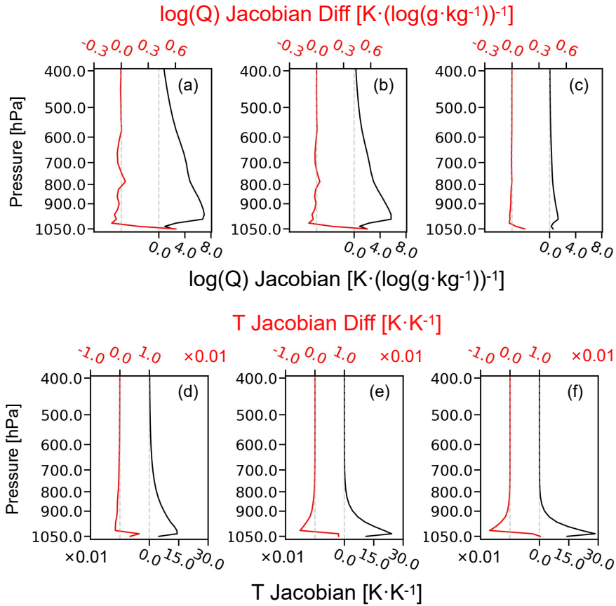
Figure 3. (a), (b) and (c): Water vapor Jacobian analysis for channels 3, 6 and 10 of HATPRO. Water vapor Jacobian based on mode 2 is presented as black lines and Jacobian differences between two interpolation modes (mode 2 minus mode 1) are presented as red lines. (d), (e) and (f): Same as (a), (b) and (c) but for temperature Jacobian analysis in different channels. The focus is on channel 11, channel 12, and channel 14 of HATPRO. RT simulations are performed under the 6th profile in the 54L UMBC 48-profile dataset. Observed zenith angle is set to 0^\circ .
