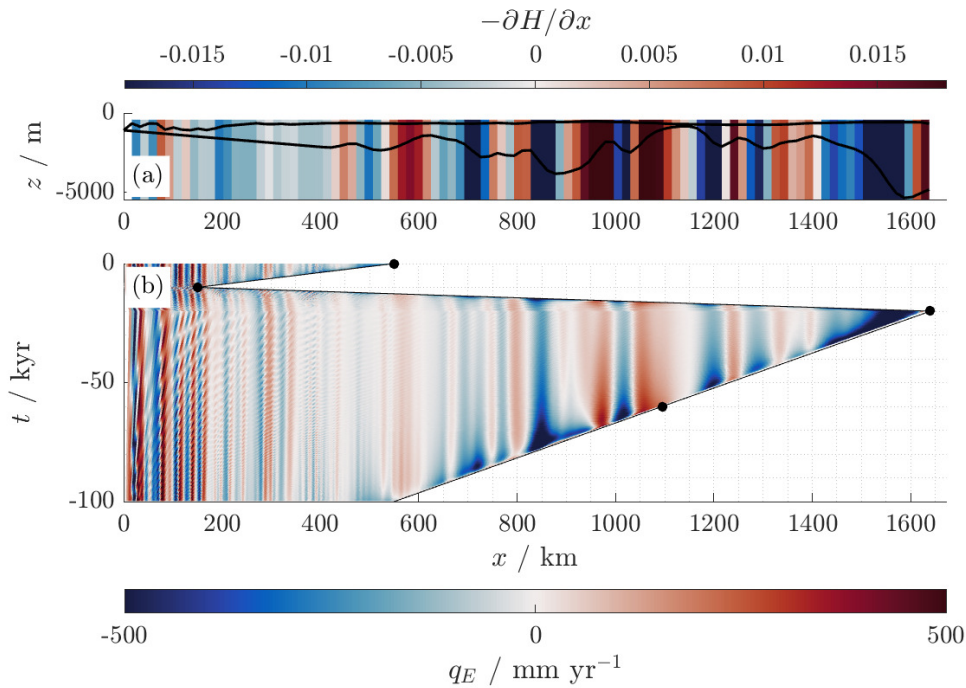
Figure 11. (a) Basement geometry b(x) and S(x) , coloured according to -\partial H/\partial x . (b) Space-time plot of q_E(x, t) , with red corresponding to q_E(x, t) > 0 (exfiltration) and blue to q_E < 0 (infiltration). Values with |q_E| > 500 \text{ mm yr}^{-1} are plotted using the same colours as \pm 500 . Parameters are as listed in Tables 1 and 2, with \alpha = 5 and k = 3 \times 10^{-12} \text{ m}^2 .
