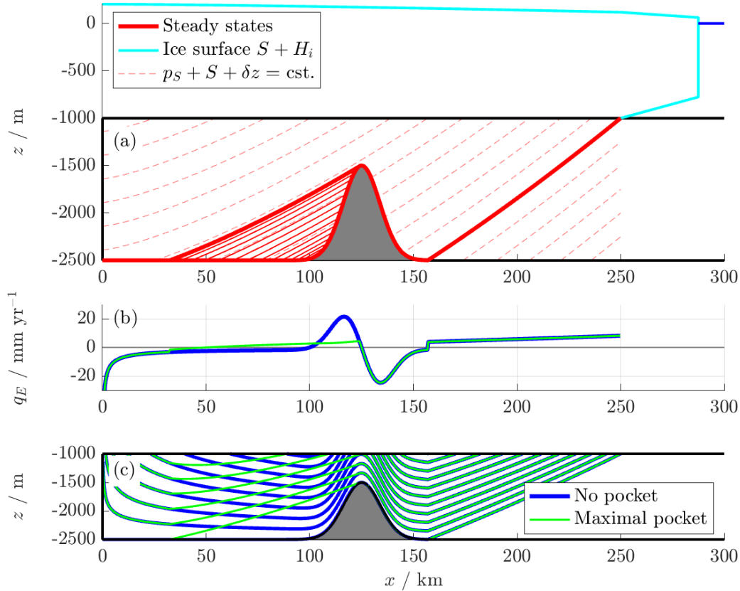
Figure 4. (a) A case with infinitely many possible “pocket” steady states, with the criteria (42) illustrated. (b) Freshwater exfiltration and (c) streamlines, with no pocket and the largest possible pocket. Parameters are as listed in Tables 1 and 2, with k = 10^{-12} \text{ m}^2 K = 0.41 and \alpha = 0.05 .
