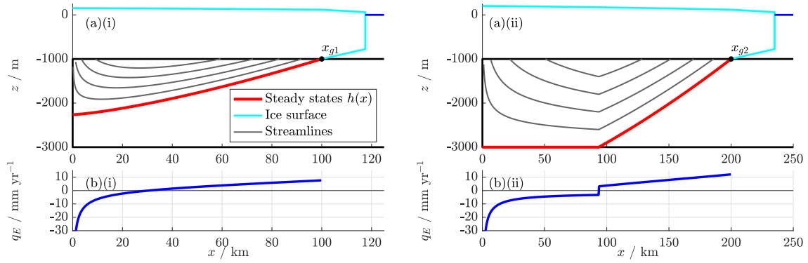
Figure 2. (a) Interface s(x) and (b) exfiltration flux q_E , for (i) “lens” and (ii) “nose” steady states arising from different grounding line positions x_{g1} and x_{g2} , for a uniform depth aquifer with b = -3000 m, S = -1000 m. Parameters are as listed in Tables 1 and 2, with k = 10^{-12} m 2 ( K = 0.41 ) and \alpha = 0.1 .
