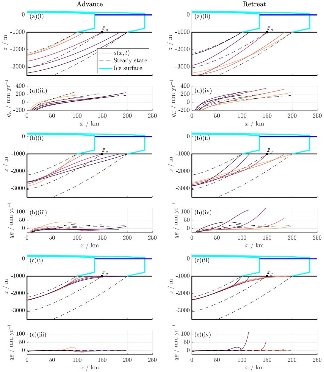
Figure 3. Stable periodic solution for s(x, t) during (i) advance and (ii) retreat, and q_E(x, t) during (iii) advance and (iv) retreat, with periodic grounding line forcing given by (38), for (a) K = 10 (high permeability) (b) K = 1 (moderate permeability) (c) K = 0.1 (low permeability). Instantaneous steady states are plotted for x_g = \bar{x}_g, \bar{x}_g \pm \Delta x_g . Parameters are as listed in Tables 1 and 2 with \alpha = 0.1 . For full solutions see Supplementary Animations S1–S3.
