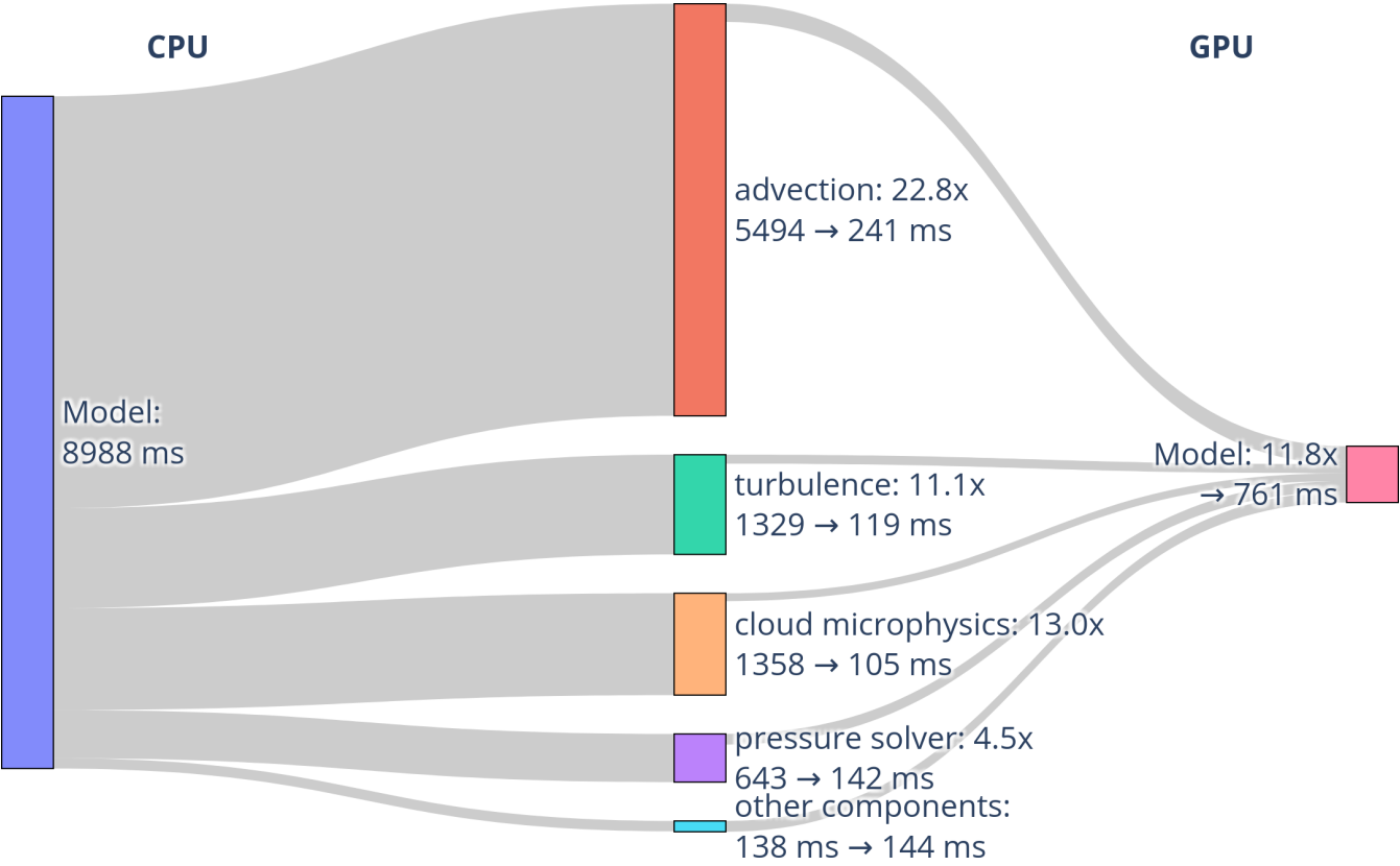
Figure 3. Sankey diagram showing the mean runtime per time step achieved on a single Adastr node for the code running on CPU on the left and running on GPU on the right. Results are shown for the 256×256×128 configuration using the FFT pressure solver.
