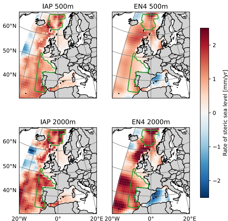
365 Figure A1: Maps of rate of vertically integrated steric sea level change in mm per year from the surface to 500m depth (upper row) and from the surface to 2000m depth (lower row). Left column is for IAP and right column for EN4. Green contours indicate the Norwegian Sea and the Extended Bay of Biscay regions.
