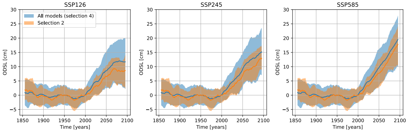
250 Figure 5: Time series of ODSL for the full CMIP6 model ensemble (blue) and for the selection of 13 plausible models based on observations (selection 2, orange). A running average of 10 years is applied. The means and 17 th to 83 rd percentile ranges are shown.
