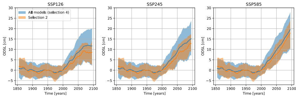
Figure 5: Time series of ODSL for the full CMIP6 model ensemble (blue) and for the selection of 12 plausible models based on observations (orange). A running average of 10 years is applied. The means and 17 th to 83 rd percentile ranges are shown.
