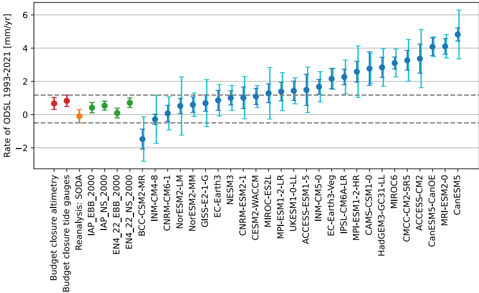
245 Figure 3: Rate of ODSL over the period 1993-2021 obtained from different observational methods and CMIP6 models after wind correction (blue). The slopes for CMIP6 models are computed from the historical experiment up to 2014 and SSP2-4.5 from 2015 to 2021. Budget closure based on tide gauge and satellite altimetry data (red), SODA ocean reanalysis (yellow), steric sea level in the top 2000 meters of the ocean from two different temperature and salt databases (IAP, EN4) and two different regions (EBB, NS, see Figure 1). The horizontal dashed lines represent the upper and lower values from observational estimates used to select models. The uncertainty ranges show ± one standard deviation
