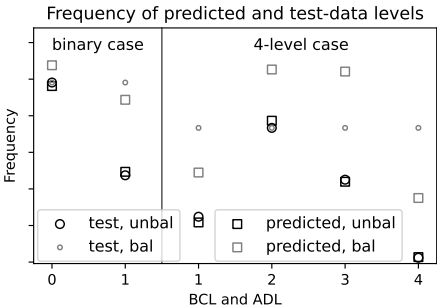
Figure 6. Confusion matrices Frequencies of occurrence of (squares) predicted and (circles) test-data danger levels for the random forest classification with respect to the unbalanced test data for (a)left the binary case with binary-case levels (BCL) and (b)right the 4-level case with avalanche danger levels (ADL). The values on the diagonals correspond to Shown are both the recall scores shown in Tables 5 (black) unbalanced and 3, respectively. For the confusion matrices with respect to the (gray) balanced test data see Fig. S9 in the supplementary information. For the corresponding confusion matrices of the artificial neural network see Fig. S1.
