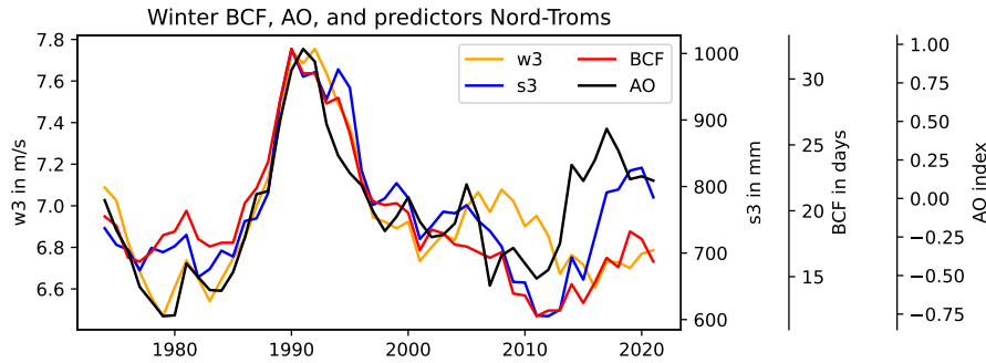
Figure 9. Binary-case avalanche-activity-frequency BCA-BCF (red), 3-day mean wind speed (w3, orange), and 3-day sum of new snow (s3, blue) in Nord-Troms and Arctic Oscillation (AO) index (black). The values correspond to 7-year rolling means.
