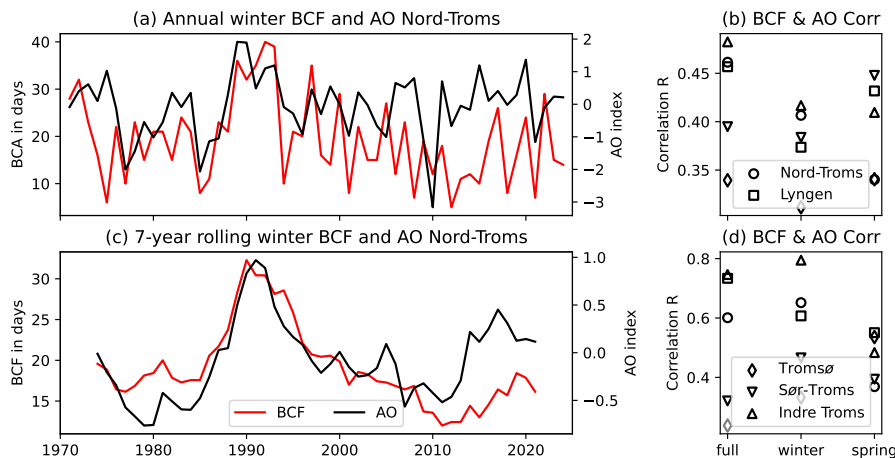
Figure 8. (a) Annual winter hindcast of binary-case avalanche activity frequency (BCA BCF, red) and Arctic Oscillation (AO) index (black) for Nord-Troms. (b) Correlation coefficients of full-season, winter, and spring BCA BCF with AO index for all regions. (c) and (d) are the same as (a) and (b), respectively, but for 7-year rolling means. Black and gray colours in (b) and (d) indicate p values smaller and larger 0.05, respectively, based on a Wald test with a t distribution. See Fig. S13 for a comparison of BCF and North Atlantic Oscillation (NAO).
