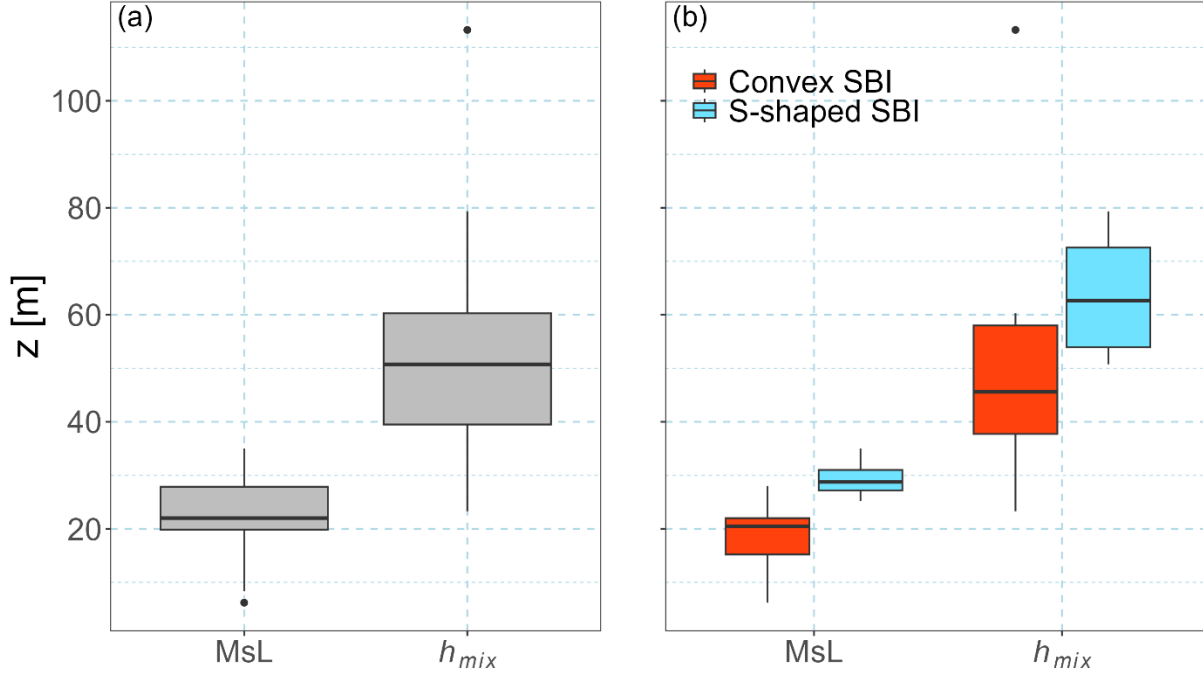
Figure 7 (a) Box plots of the mixed sublayer (MsL) height and mixing layer height ( h_{mix} ) for cases of the stable boundary layer. (b) Same as (a) but cases of convex and ‘s-shaped’ SBI are shown separately. The thick horizontal line represents the median, the box the interquartile range and the whiskers’ lengths are equal to 1.5 time the interquartile range.
