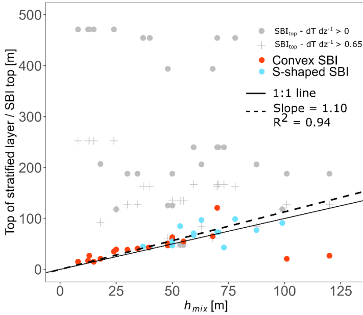
Figure 8 Comparison between h_{mix} and the top of the stratified layers and SBI top. The top of the stratified layer for convex cases is the top of the first layer (strongest temperature gradient) and top of the second layer for ‘s-shaped’ cases, indicated by the color of the dots. Grey dots (crosses) indicate SBI top retrieval with a dT/dz threshold of 0^{\circ}\text{C } 100\text{m}^{-1} ( 0.65^{\circ}\text{C } 100\text{m}^{-1} ). The full line represents the 1:1 diagonal and the dashed line represents the slope of a linear regression fit through the data points corresponding to stratified layer heights.
