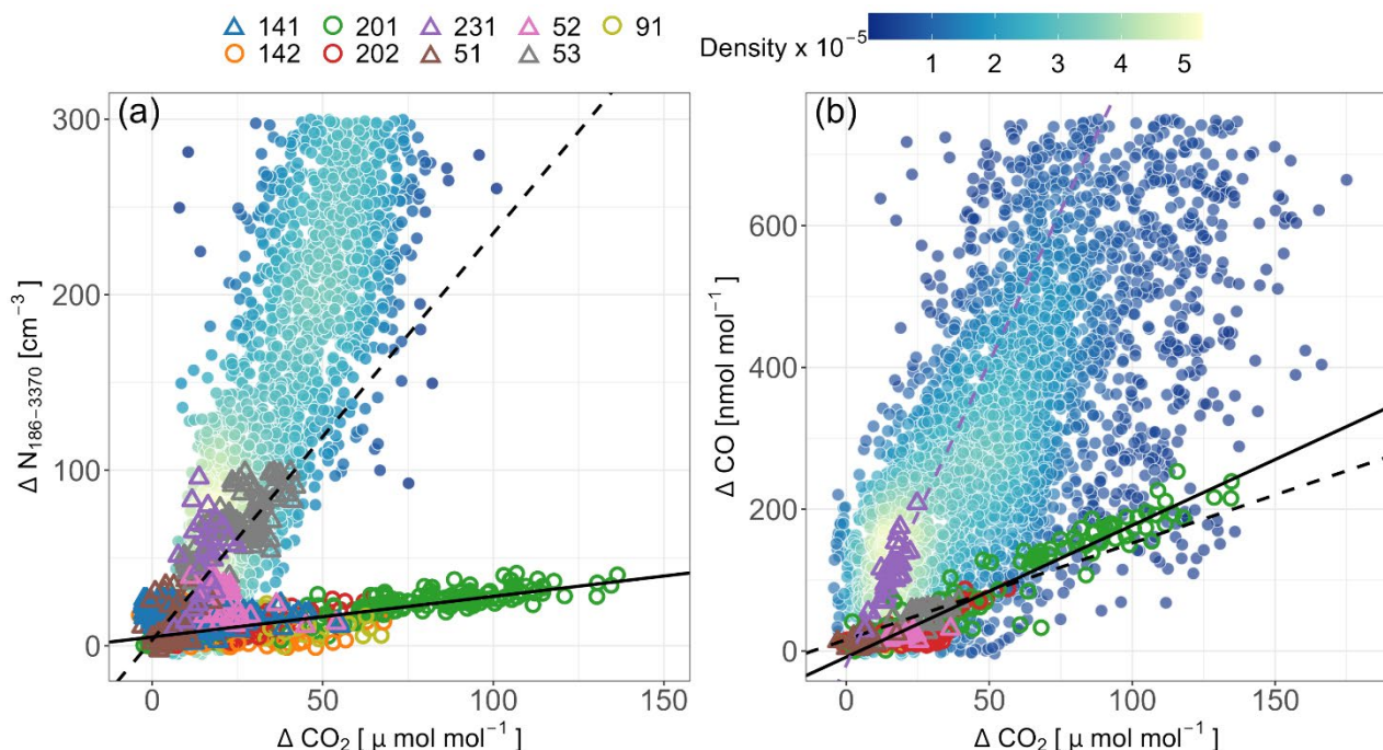
935 Figure 13 Tracer-tracer relationship of measured elevated plumes compared to ground-based observations downtown Fairbanks. The different tracers are expressed as concentration enhancements between the measured value in the plume and the average concentration of the WPBL (outside the plume). Circles represent data points from UAF C plumes. Triangles represent data points from other plumes. The full lines represent a linear regression through data points corresponding to UAF C plumes (coal-fired power plant). The dashed black lines are for the other plumes of uncertain origin (likely coal- and/or diesel-powered power plants). 940 The purple dashed line likely corresponds to a pollution plume originating from Chena ridge (likely from domestic heating). Dots in the back correspond to tracer-tracer relationships from ground-based measurements at CTC. The color-coding corresponds to the density of observations.
