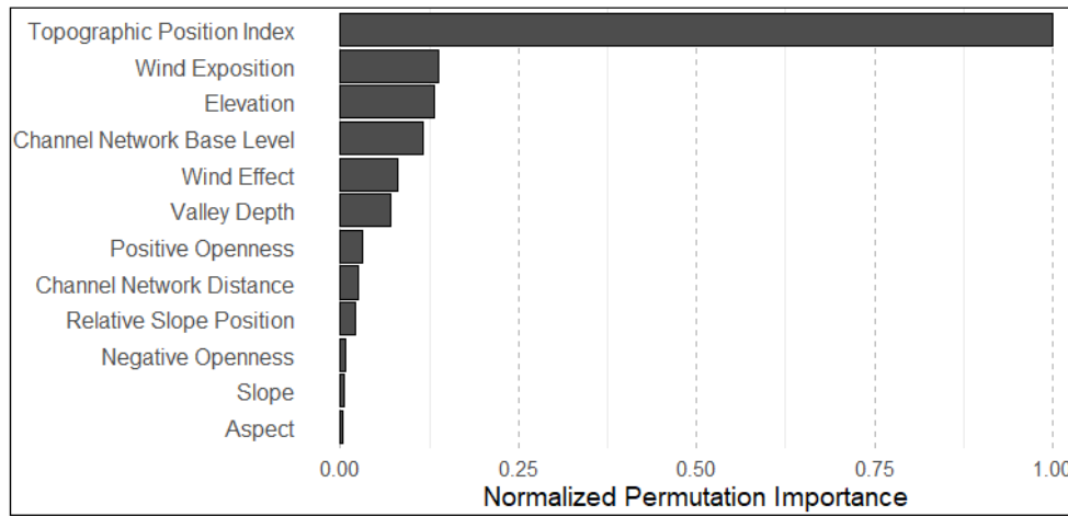
Figure 7. Overview of normalized mean Permutation Importance values from RF modeling over 100 iterations.
