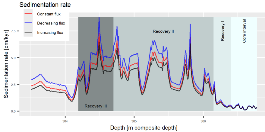
Figure 6. Median sedimentation rate and condensation in the stratigraphic domain for the three scenarios defined.
