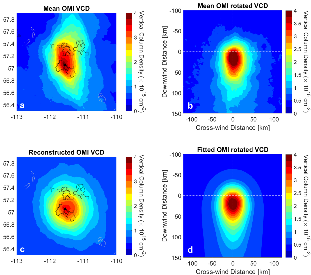
Figure 2. Summary of the point source emissions procedure using 2005–2022 OMI \text{NO}_2 VCDs. (a) Mean OMI VCD over the surface mining region of the oil sands. The black lines denote the different mining operations; (b) mean OMI VCD after rotation showing plume-like structure; (c) Reconstructed spatial distribution using EMG plume and fitted parameters; (d) Fit to rotated VCD using 2D EMG plume function, with fitted parameters of E=69.7 \text{ kt}[\text{NO}_2]/\text{yr} , \tau = 3.2 hours, and \sigma = 20.6 km. The black triangle in the panels (a) and (c) show the reference location used in the emissions retrieval and corresponds to the (0, 0) point in panels (b) and (d).
