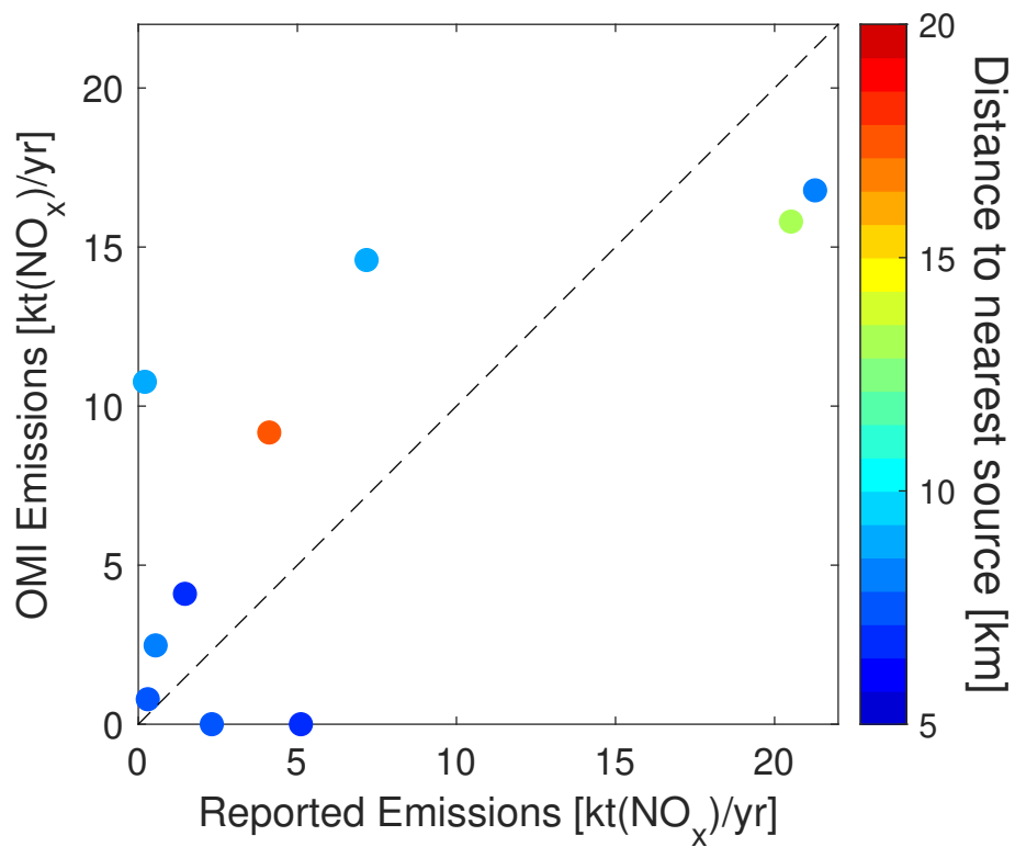
Figure F3. Comparison of reported and OMI-derived NO x emissions derived for individual mining operations considering the years 2010–2020, colour-coded according to proximity the their nearest neighbour.
