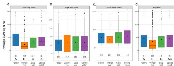
Figure 2. Mean soil mineral nitrogen (SMN) during the different cropping phases. Mean SMN ± SD (n=12 for rye treatment in the sugar beet, winter wheat and all phases together, n=16 for all other treatments). Horizontal lines represent the median, large dots and numbers at the bottom show the mean. Uppercase letters indicate significant differences of Z-standardized Nmin values between the treatments (p<0.05).
