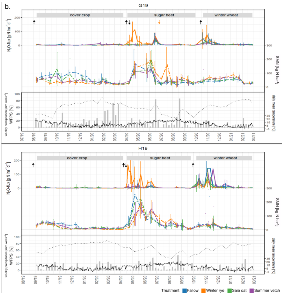
Figure 1. Dynamics of \text{N}_2\text{O} flux rates and soil mineral nitrogen (SMN) contents, presented as mean \pm SD ( n=4 ). Seasonal changes in topsoil water-filled pore space (WFPS%, dotted black line), daily mean air temperature (continuous black line) and weekly precipitation (gray bars) for Göttingen (upper plot) and Hohenheim (lower plot) throughout the different cropping phases for various CC treatments in (a) 2018 trials and (b) 2019 trials. Upward arrows mark soil cultivation events, while downward arrows signify N fertilization of sugar beets.
