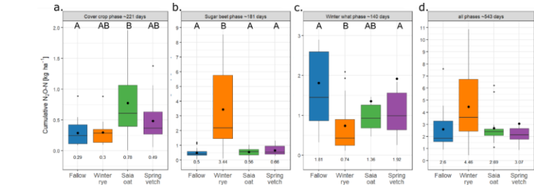
Figure 3. Cumulative N 2 O emissions across the different cropping phases. Mean \pm SD (n=12 for rye in sugar beet and winter wheat phases and all phases combined; n=16 for all other treatments). Horizontal lines represent the median, large dots and numbers at the bottom show the mean. Uppercase letters indicate significant differences of Z-standardized cumulative N 2 O emission values between the treatments (p<0.05).
