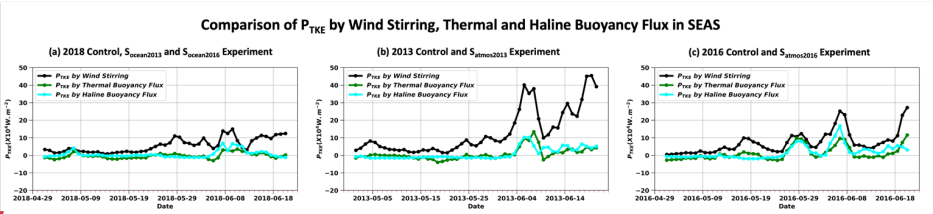
Fig. 13 Comparison of P_{TKE} by wind, thermal, and haline buoyancy flux averaged in the SEAS (72-76°E and 7-13°N) from May 1 to June 20. The values are shown here after multiplying 10^4 .
