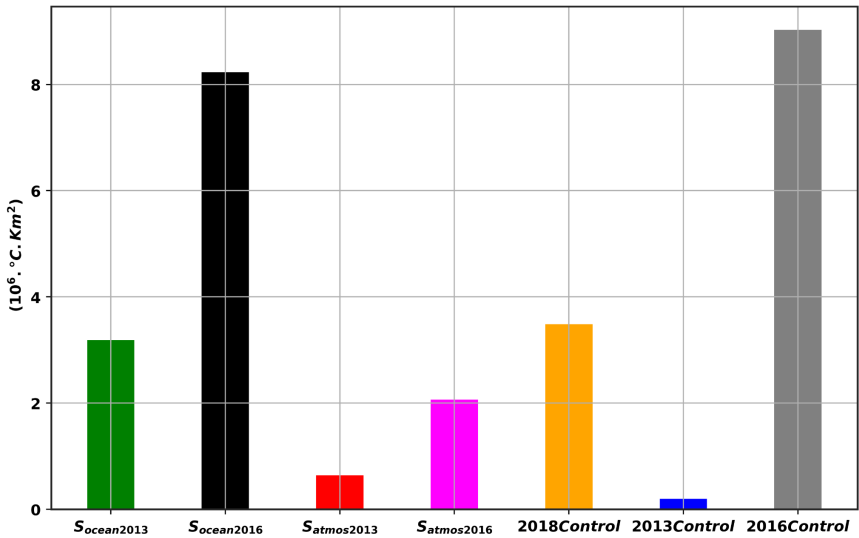
465 Figure 12: A comparison of the MWP intensity index in all three experiments during the respective mature phase days in different years. In S_{ocean2013} , S_{ocean2016} , S_{atmos2013} , 2013 control experiment, and 2018 control experiment, the mature day was May 20. In the S_{atmos2016} and 2016 control experiments, the mature day was May 4.
