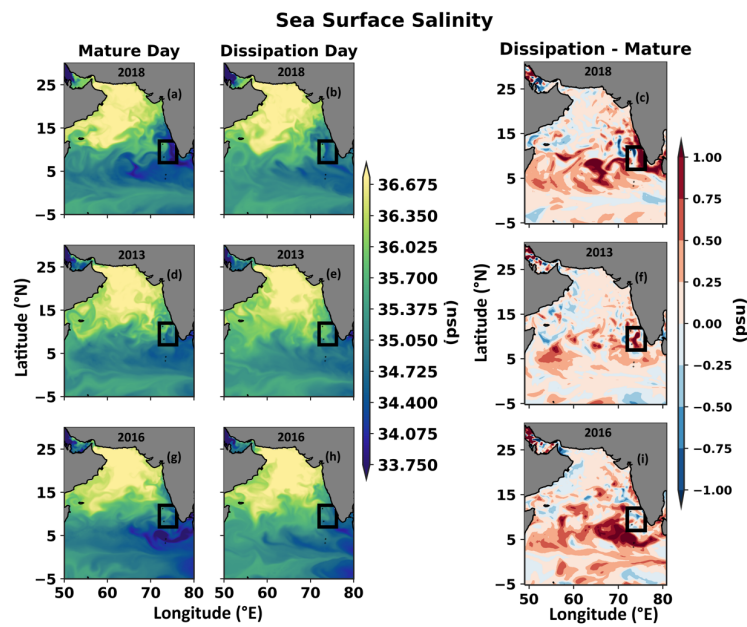
370 Figure 7: Comparison of sea surface salinity on mature and dissipation days in 2018 (a-c) (MWP strength close to climatology), 2013 (d-f) (MWP was absent), and 2016 (g-i) (MWP was intense). (c), (f), and (i) show the distinction between dissipation and mature day. The MWP's mature days are May 20, 2018, 2013, and May 4, 2016. The MWP's dissipation days were June 8, 2018, 2013, and June 6, 2016. The black box is the core MWP region.
