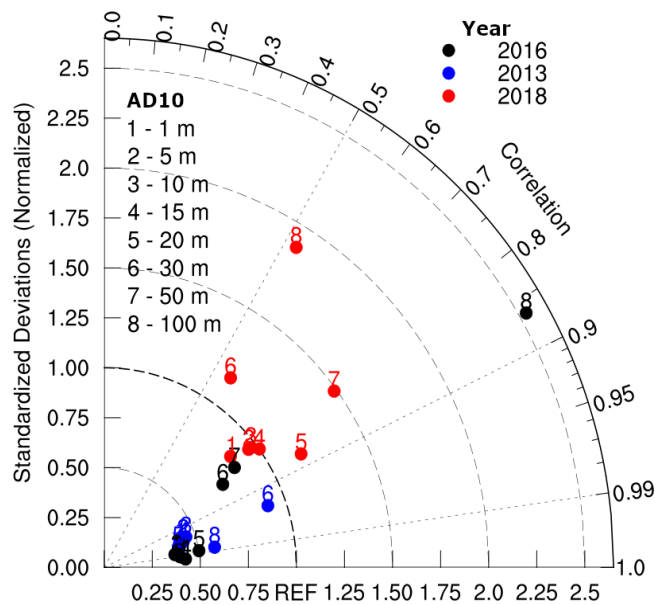
Figure 5: Taylor diagram showing the temporal correlation and standard deviations of the model simulated temperature profile from the three years of model experiments with respect to measurements at the buoy AD10.
