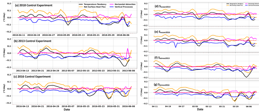
Figure 11: Area averaged (72- 76°E and 7-13°N, i.e., the white box shown in Fig. 1) mixed layer heat budget for three control ((a) 2018 control experiment, (b) 2013 control experiment, and (c) 2016 control experiment) and four sensitivity experiments ((d) Soccean2013, (e) Soccean2016, (f) S atmos 2013, and (g) S atmos 2016). In the sensitivity experiments, the oceanic and atmospheric conditions have been changed to various years; thus, only the day and month are kept on the x-axis (d to g). For better understanding, the mixed layer heat budget is shown from April 10 th , even though we have considered April 1 st to April 30 th as the spin-up time.
