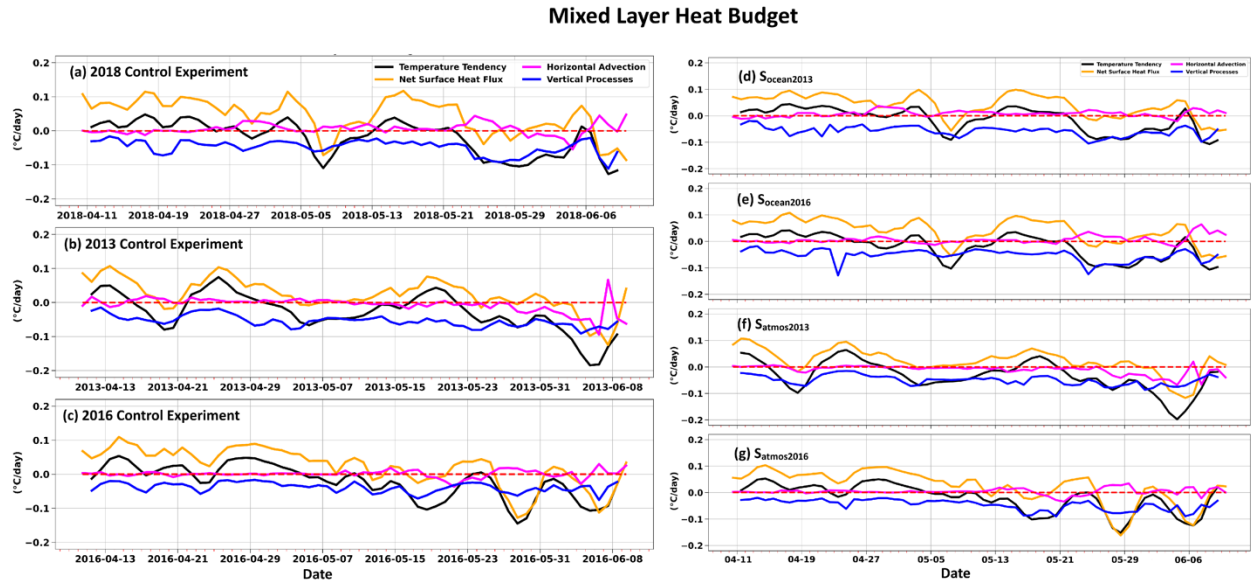
Fig R 4 Area averaged (72– 76°E and 7–13°N) mixed layer heat budget for three control ((a) 2018 control experiment, (b) 2013 control experiment, and (c) 2016 control experiment) and four sensitivity experiments ((d) Socean2013, (e) Socean2016, (f) S Atmos2013, and (g) S Atmos2016). In the sensitivity experiments, the oceanic and atmospheric conditions have been changed to various years; thus, only the day and month are kept on the x-axis (d to g).
