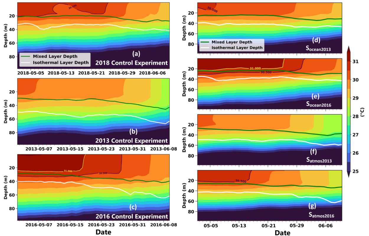
Fig R 1 Area averaged (72- 76°E and 7-13°N, i.e., the core MWP region) vertical temperature for three control ((a) 2018 control experiment, (b) 2013 control experiment, and (c) 2016 control experiment) and four sensitivity experiments ((d) Socean2013 , (e) Socean2016 , (f) S_atmos2013 , and (g) S_atmos2016 ). In the sensitivity experiments, the oceanic and atmospheric conditions have been changed to various years; thus, only the day and month are kept on the x-axis.
