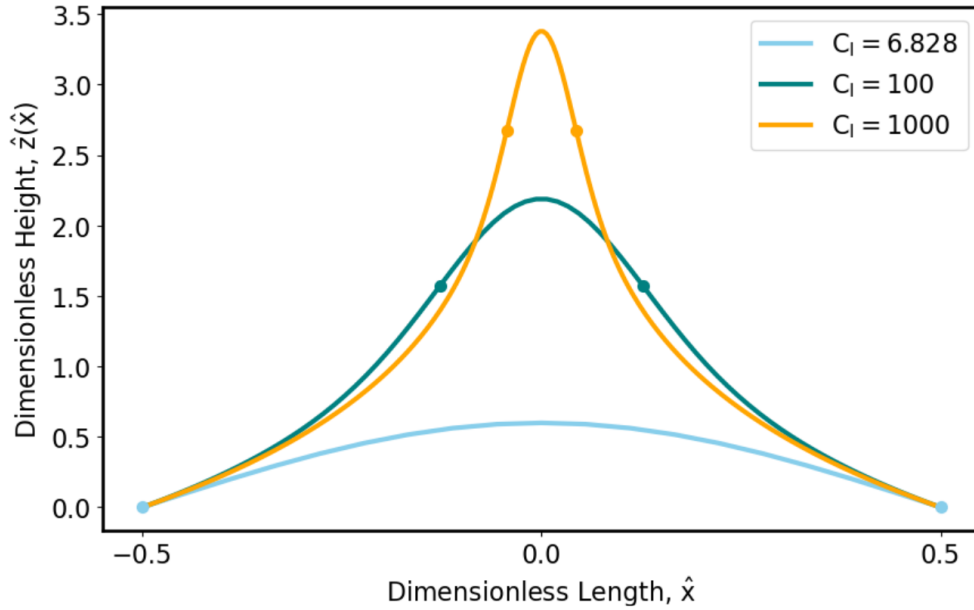
Figure 1. Equation 3 solved for various values of C_I . As noted in Anand et al. (2023), concave-down profiles are locally preserved near \hat{x} = 0 for asymptotically large values of C_I . Inflection points are plotted with dots. The value C_I \approx 6.828 sets the distance between the inflection points equal to the boundary length.
