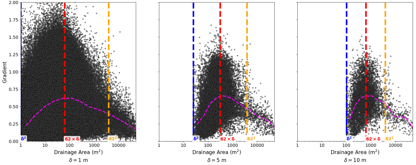
Figure 7. Log-log plot of slope by drainage area for Gabilan Mesa, resampled across 1, 5, and 10 meter pixels, as shown in Fig. 8. The binned median is plotted in a magenta dashed line. The characteristic length is 62 m. The minimum drainage area, corresponding to topographic maxima is \delta^2 . The drainage area of the inflection point is 62\delta^2 . Channel heads have the characteristic area of contributing drainage area which is resolution-independent.
