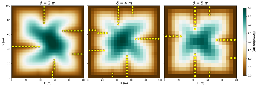
Figure 4. Computational results varying \delta for U = 1e-3 \text{ m yr}^{-1} , D = 5e-2 \text{ m}^2 \text{ yr}^{-1} , K = 5e-4 \text{ yr}^{-1} . Nodes with drainage area exceeding a = \frac{r^2}{\delta} are shown with yellow dots. Varying \delta with \frac{r}{\ell} constant produces similar results. With decreasing \frac{r}{\delta} , maximum elevation decreases, since topographic maxima have specific drainage area \delta . This presents a possible benefit for subtracting \delta from a , thus counting the number of links (Rodríguez-Iturbe et al., 1997). We forgo this approach for simplicity.
