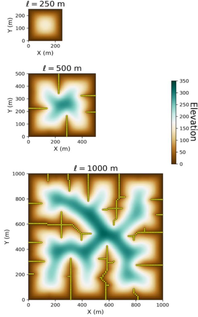
Figure 3. Computational simulation results varying \ell for \delta = 10 m, K = 2.5e-5 yr ^{-1} , D = 7e-2 m ^2 yr ^{-1} , U = 3.6e-3 m yr ^{-1} . The corresponding channelization indices, CI = \frac{\ell^2 K}{D} , are approximately 22, 89, and 357. These simulations preserve the dimensionless group \frac{r}{\delta} , the ratio of the characteristic length to the pixel width. Larger values of CI , given the same r value, imply a resized boundary length, \ell . Channels are highlighted with yellow dots for A \geq r^2 .
