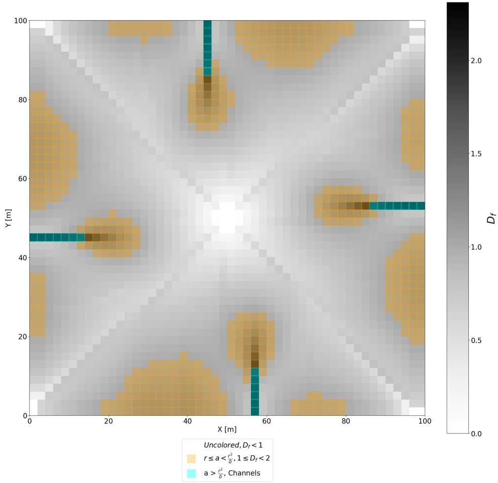
Figure 6. Simulation result for U = 1e-3 \text{ m yr}^{-1} , D = 5e-2 \text{ m}^2 \text{ yr}^{-1} , K = 2.5e-4 \text{ yr}^{-1} , \delta = 2 \text{ m} , and \ell = 100 \text{ m} , plotted according to the fractal dimension, D_f (Eq. 12). Channel heads, with drainage area r^2 , have dimension two. Colluvial valleys correspond to 1 < D_f < 2 . River segments have dimension two when accounting for channel width.
