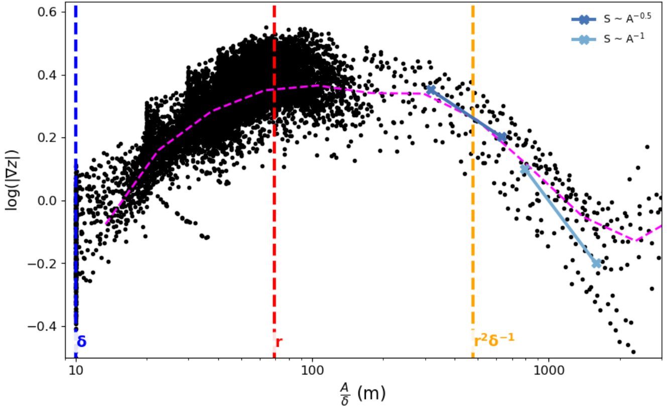
Figure 2. Slope-specific drainage area plot for the simulated topography shown in Fig. 3 for \ell = 1000 m, \delta = 10 m, K = 2.5e-5 yr ^{-1} , D = 7e-2 m ^2 yr ^{-1} , U = 3.6e-3 m yr ^{-1} . The binned median slope is plotted in magenta. The specific drainage area a = r , shown with the red line, has the steepest slope. The specific drainage area value \frac{r^2}{\delta} , shown in orange, represents the transition to fluvial power-law scaling, with slope decreasing steadily with contributing area. This value is resolution independent as an area, but not as a specific drainage area, which has the fundamental dimension of length.
