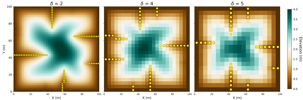
Figure 4. Computational results varying \delta for U = 1e-3m yr^{-1} , D = 5e-2m^2 yr^{-1} , K = 5e-4yr^{-1} . Nodes with drainage area exceeding a = \frac{r^2}{\delta} are shown with yellow dots. Varying \delta with \frac{r}{\ell} constant produces similar results. With decreasing \frac{r}{\delta} , maximum elevation decreases, since topographic maxima have specific drainage area \delta . This presents a possible benefit for subtracting \delta from a , thus counting the number of links (Rodríguez-Iturbe et al., 1997). We forgo this approach for simplicity.
