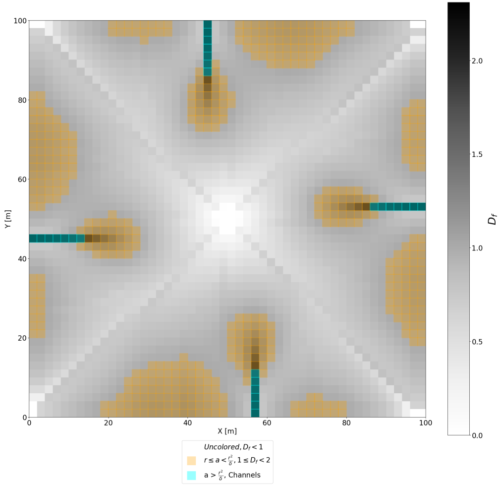
Figure 6. Simulation result for U = 1e-3m\text{yr}^{-1} , D = 5e-2m^2\text{yr}^{-1} , K = 2.5e-4\text{yr}^{-1} , \delta = 2 , \ell = 100 plotted according to the fractal dimension, D_f (Eq. 12). Channel heads, with drainage area r^2 , have dimension two. Colluvial valleys correspond to 1 < D_f < 2 . River segments have dimension two when accounting for channel width.
