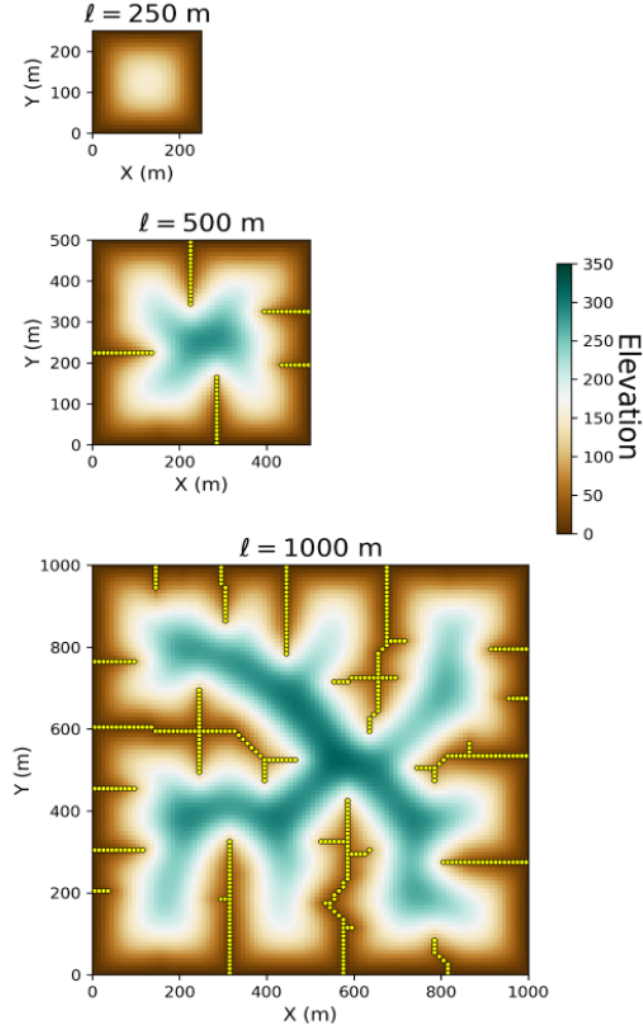
Figure 3. Computational simulation results varying \ell for \delta = 10 , K = 2.5e - 5yr^{-1} , D = 7e - 2m^2yr^{-1} , U = 3.6e - 3myr^{-1} . The corresponding channelization indices, CI = \frac{\ell^2 K}{D} , are approximately 22, 89, and 357. These simulations preserve the dimensionless group \frac{\tau}{\delta} , the ratio of the characteristic length to the pixel width. Larger values of C_I , given the same r value, imply a resized boundary length, \ell . Channels form for A = r^2 , shown are highlighted with yellow dots for A \geq r^2 .
