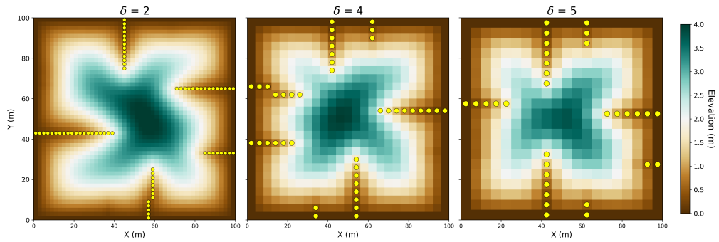
Figure 4. Computational results varying \delta for U = 1e-3\text{myr}^{-1} , D = 5e-2\text{m}^2\text{yr}^{-1} , K = 2.5e-4\text{yr}^{-1} K = 5e-4\text{yr}^{-1} . Nodes with drainage area exceeding a = \frac{r^2}{\delta} are shown with yellow dots. Varying \delta with \frac{r}{\ell} constant produces similar results. With decreasing \frac{r}{\delta} , maximum elevation decreases, since topographic maxima have specific drainage area \delta . This presents a possible benefit for subtracting \delta from a , thus counting the number of links (Rodríguez-Iturbe et al., 1997). We forgo this approach for simplicity.
