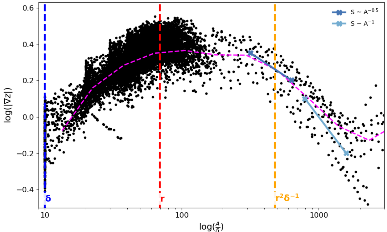
Figure 2. Slope-specific drainage area plot for the simulated topography shown in Fig. 3-3 for \ell = 1000 , \delta = 10 , K = 2.5e - 5yr^{-1} , D = 7e - 2m^2yr^{-1} , U = 3.6e - 3myr^{-1} . The binned median slope is plotted in magenta . The specific drainage area a = r , shown with the red line, has the steepest slope. The specific drainage area value \frac{r^2}{\delta} , shown in orange, represents the transition to fluvial power-law scaling, with slope decreasing steadily with contributing area. This value is resolution independent as an area, but not as a specific drainage area, which has the fundamental dimension of length .
