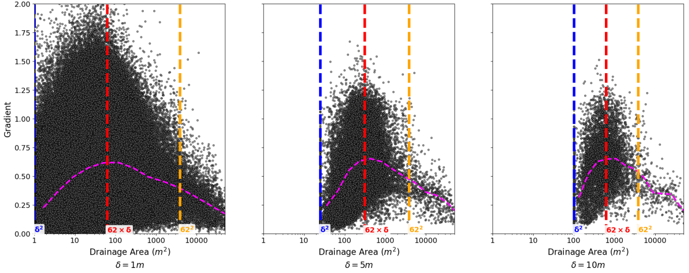
Figure 7. Log-log plot of slope by drainage area for nodes in Fig. 8 Gabilan Mesa, corresponding to resampled across 1, 5, and 10 meter pixels, as shown in Fig. 8 . The binned median is plotted in a magenta dashed line. The characteristic length is 62m. The minimum drainage area, corresponding to topographic maxima is \delta^2 . The drainage area of the inflection point is 62\delta m^2 62\delta m^2 . Channel heads have the characteristic area of contributing drainage area which is resolution-independent.
