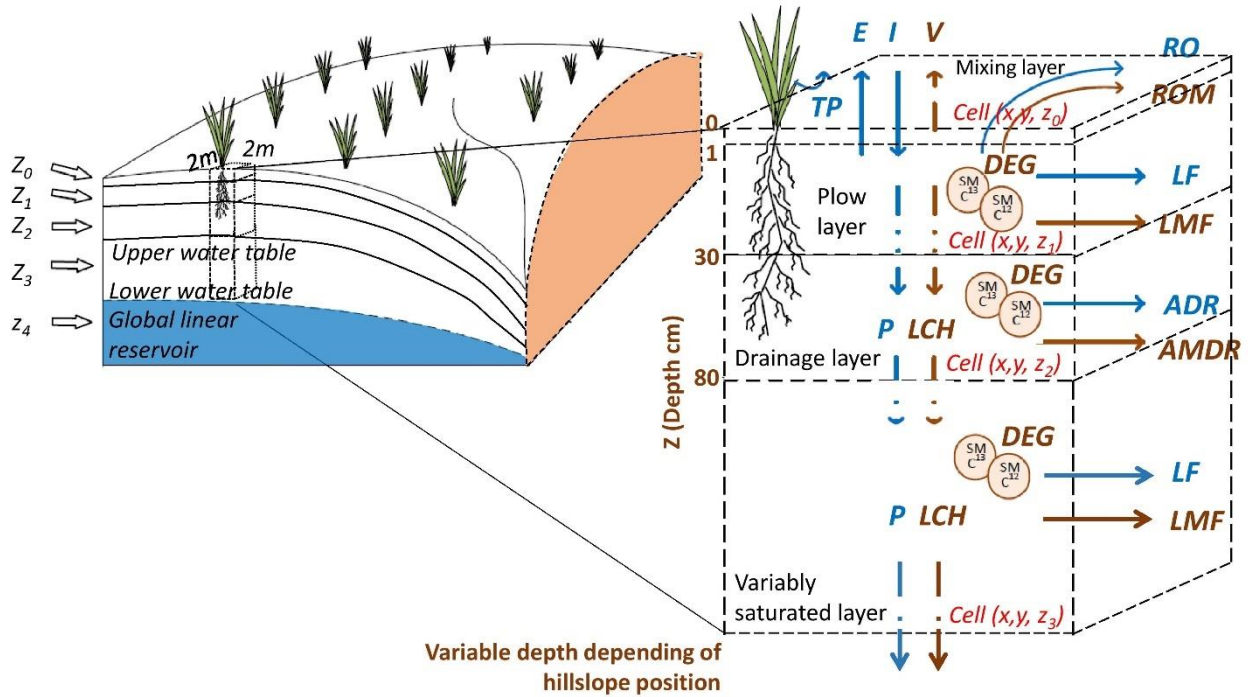
Figure 2: Conceptual representation of the five-layer ( z_0 to z_4 ), spatially distributed hydrological and reactive transport model PiBEACH, employing a 2 \times 2 m raster resolution and variable depths depending on soil layers, from z_0 to z_3 . Hydrological processes include evaporation ( E ), transpiration ( TP ), percolation ( P ), volatilization ( V ), runoff ( RO ), lateral flow ( LF ), and artificial drainage ( ADR ). Pesticide mass transfer processes include volatilization ( V ), runoff mass ( ROM ), lateral mass flow ( LMF ), leaching ( LCH ), mass transfer via artificial drainage ( AMDR ), and degradation ( DEG ) with isotope fractionation ( SM^{13}C and SM^{12}C ).
