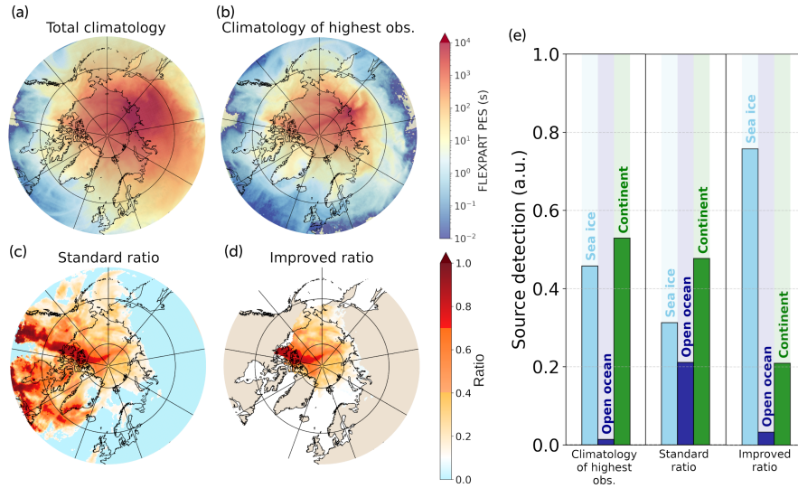
Figure 6. Panel of backtrajectory-FPES visualisations and analysis for the sea ice tracer at the Tiksi station. (a) and (b) are the climatologies of respectively the total backtrajectories-FPES and the-trajectories-those associated to-with the 10 % highest observations ( S_h^{10} ). (c) and (d) are the ratio maps of the two versions of the ratio method ( R_h^{10} for respectively the standard and improved versions). (e) is the quantification of the detection results for the climatology associated to-with the highest observation and for both versions of the ratio method.
