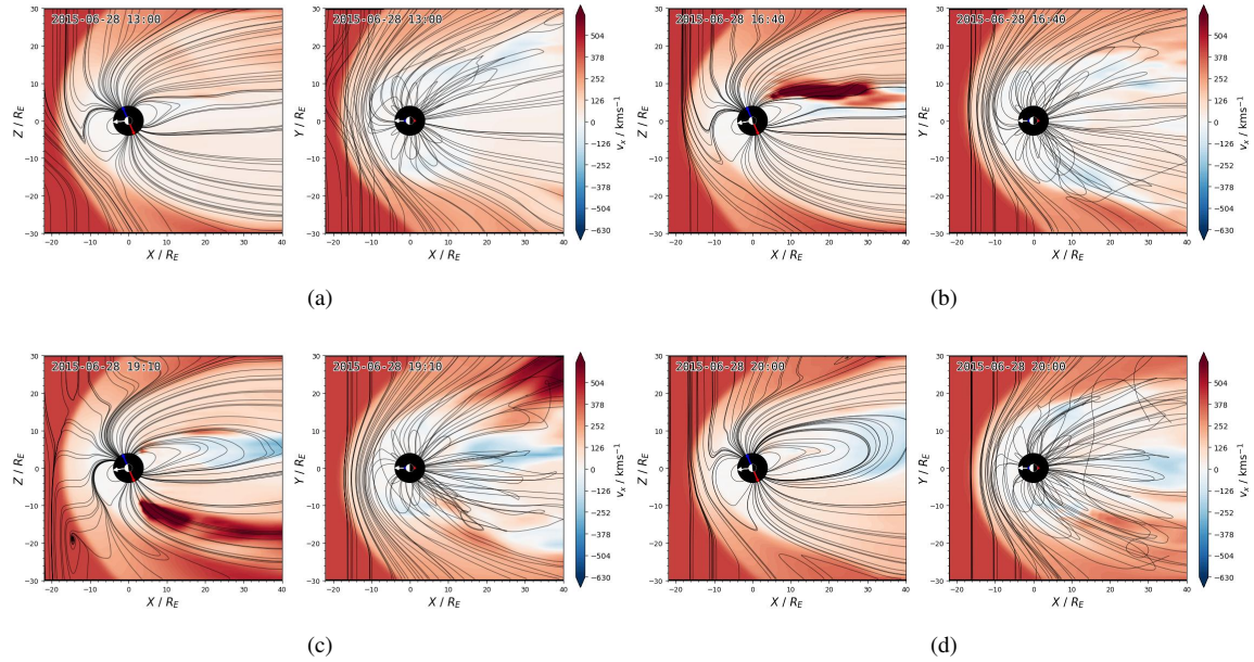
Figure 6. Snapshot of solar-wind-flow velocity from the MHD simulation with Gorgon-Space. It depicts the arrival time of the second CME, which began on 25 June 2015 at 14:52 and reached Earth on 28 June 2015 at 12:52 UT, in the noon-midnight plane. All panels are shown in GSE coordinates.
