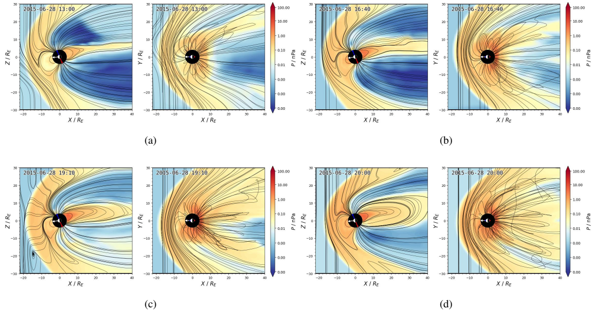
Figure 4. Snapshot of solar-wind thermal pressure from the MHD simulation with Gorgon-Space. It depicts the arrival time of the second CME, which began on 25 June 2015 at 14:53 and reached Earth on 28 June 2015 at 12:52 UT, in the noon-midnight plane. All panels are shown in GSE coordinates. Note that the X and Y axes in GSE are opposite to those in GSM.
