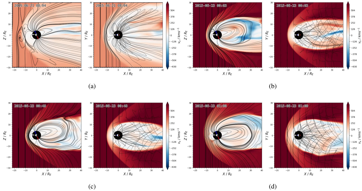
Figure 5. Snapshot of solar-wind-flow velocity from the MHD simulation with Gorgon-Space. It depicts the arrival time of the first CME, which began on 21 June 2015 at 08:02 and reached Earth on 23 June 2015 at 00:03 UT, in the noon-midnight plane. All panels are shown in GSE coordinates.
