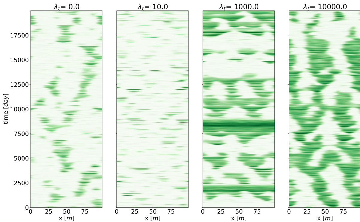
Figure 5. Four realizations of the stochastic Rietkerk model with \lambda_s = 1\text{m} . The biomass is the variable shown. Each panel shows a representative realization with different temporal autocorrelations ( \lambda_t ).
