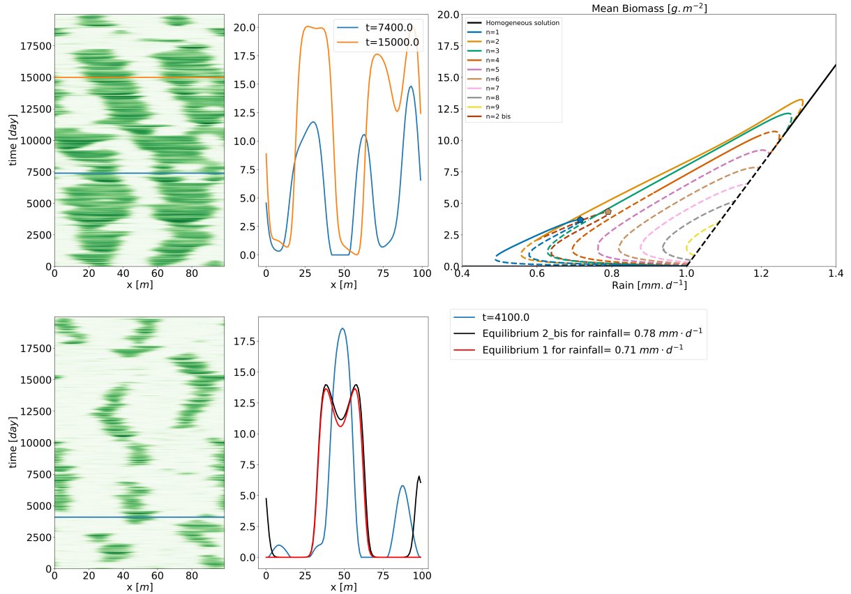
Figure 6. Two realizations of the stochastic Rietkerk model with different noises. On the top-left panel, the parameters are R = 0.8 \text{ mm d}^{-1} , \lambda_t = 1 \text{ d} and \lambda_s = 10 \text{ m} for the noise applied on the biomass, and \lambda_t = 10000 \text{ d} and spatially homogeneous for the noise applied on the surface water. On the bottom-left panel, the parameters are R = 0.8 \text{ mm d}^{-1} , \lambda_t = 1 \text{ d} and \lambda_s = 15 \text{ m} for the noise applied on the biomass, and \lambda_t = 1 \text{ d} and spatially homogeneous for the noise applied on the surface water. The three horizontal lines mark the timing of the snapshots represented on the middle panels respectively. The top-right panel gives the bifurcation diagram with two pentagons marking the position of two equilibria shown on the bottom-center panel.
