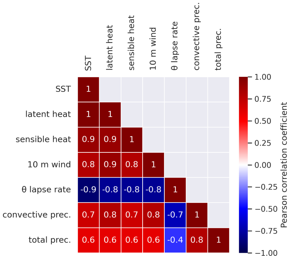
Figure 9: Pearson correlation coefficient (R) between the SST differences (Fig. 5b, CPL – STD) and the differences in the atmospheric fields analysed (Fig. 7, CPL – STD), during the extreme winter cyclones. The matrix is symmetric. \theta stand for potential temperature.
