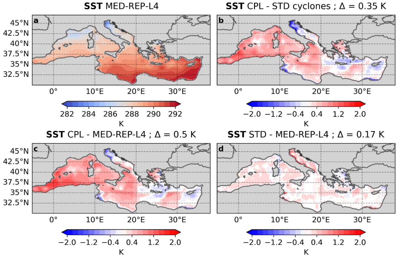
Figure 5: Maps for the SST from the MED-REP-L4 observational dataset (a), maps of difference in SST between CPL and STD for winter extreme cyclones (b), maps of the winter climatological difference in SST between CPL and MED-REP-L4 (c) and between STD and MED-REP-L4 (d). The white colour indicates no significant differences at 5 % confidence level. \Delta values represent the domain average of the differences where the values are statistically significant.
