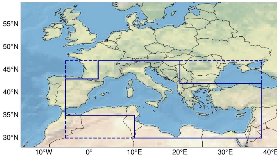
240 Figure 1: Med-CORDEX domain. Cyclones are retained if their minimum SLP tracking point is present within the area outlined by solid lines. The atmospheric fields are computed within the rectangular area outlined by dashed lines.
