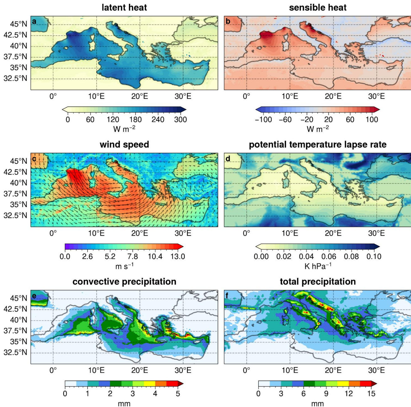
Figure 4: Maps for latent heat flux (a), sensible heat flux (b), 10 m wind speed and direction (c), potential temperature lapse rate (d), convective precipitation (e) and total (large-scale + convective) precipitation (f) from the STD simulation during winter extreme cyclones in common with CPL.
