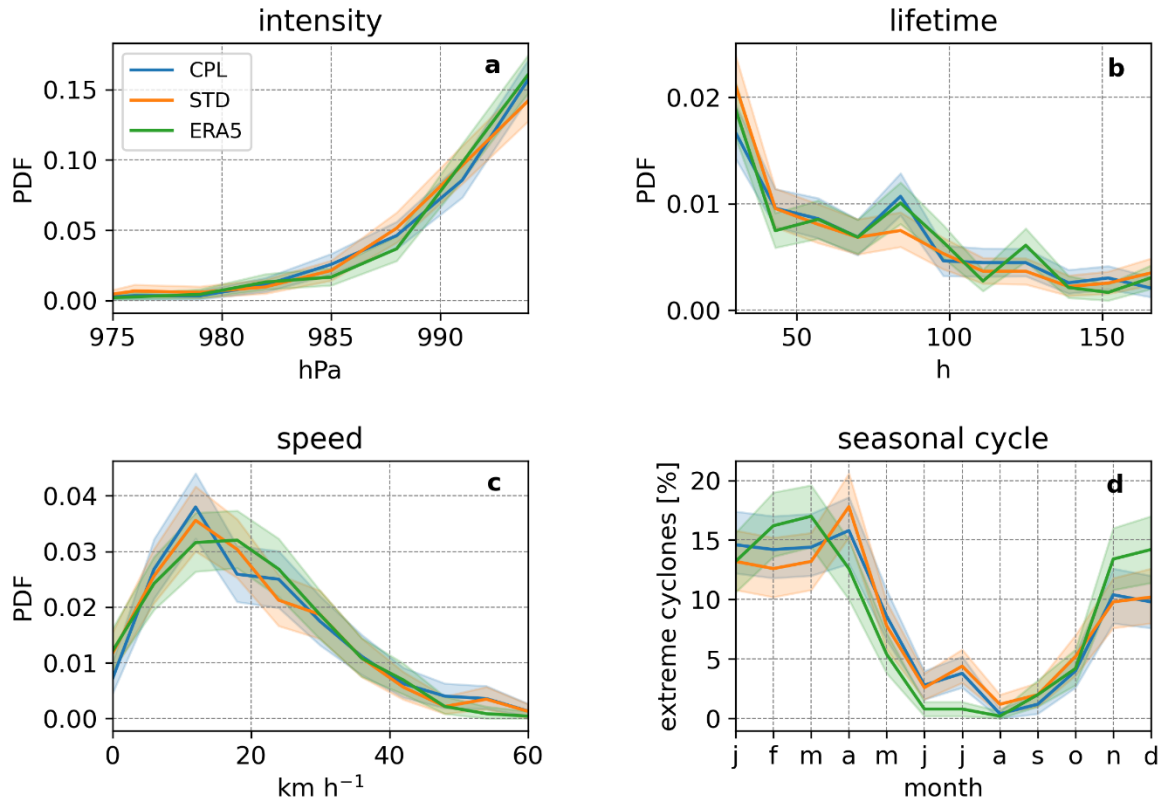
Figure 2: Statistics, intensity (a), lifetime (b) and speed (c), and seasonal cycle (d) of the 500 most intense cyclones in STD, CPL and ERA5. The colour band represent the 2.5-97.5% confidence interval within the 1000 bootstrap surrogates.
