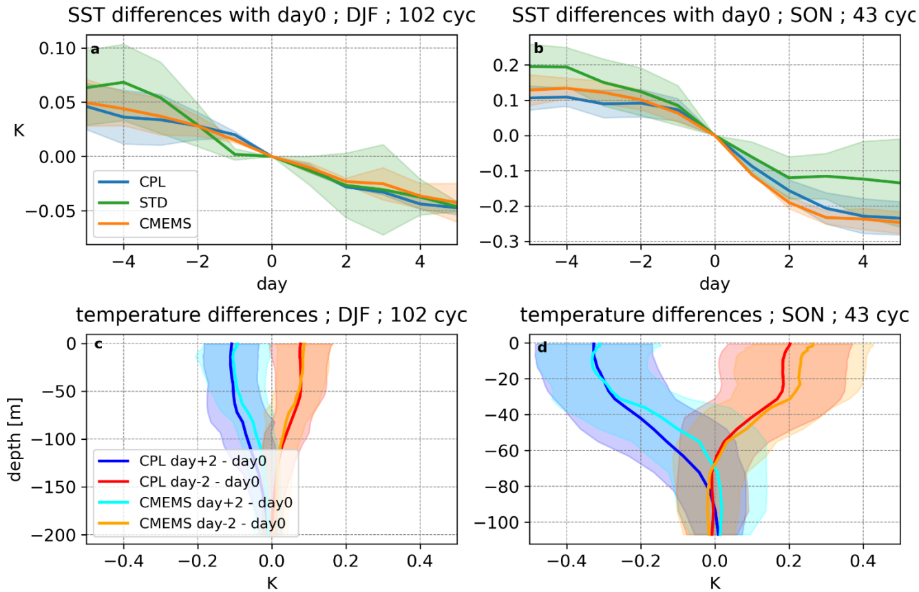
525 Figure 10: SST evolution compared with the SST on the day of the cyclone from five days before to five days after the event for CPL (blue line), STD (green line) and CMEMS MED-Currents reanalysis (orange line), averaged over the same cyclones in DJF (a) and in SON (b). The vertical profiles of the ocean temperature computed as difference between 2 days before and the day of the cyclones (similarly for 2 days after the event) for CPL (blue and red lines) and CMEMS MED-Currents (light blue and orange lines), averaged over the same cyclones in DJF (c) and in SON (d). In each figures the temperature values represent the average over a circular area with 1.5° radius, around the minimum SLP tracking point, and over the cyclones considered. The colour bands represent the confidence interval between +- 1 standard deviation of the mean of the temperature differences.
