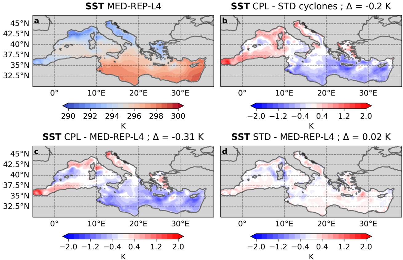
385 Figure 6: Same as figure 5, but for SON.
