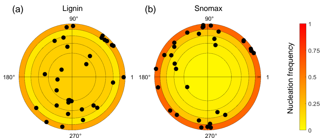
Figure 2. Onset freezing locations for droplets squeezed between two protein-repellent glass slides (a) Lignin ( 5000 \text{ mgC L}^{-1} ) and (b) literature data for filtered Snomax ( 125 \text{ mgC L}^{-1} ) from Bieber and Borduas-Dedekind (2024). The mean freezing temperatures were -20.6^\circ\text{C} for lignin and -6.3^\circ\text{C} for the filtered Snomax sample, which is in the range of the investigated concentrations. Note that the droplet volume was 0.5 \mu\text{L} for these measurements.
