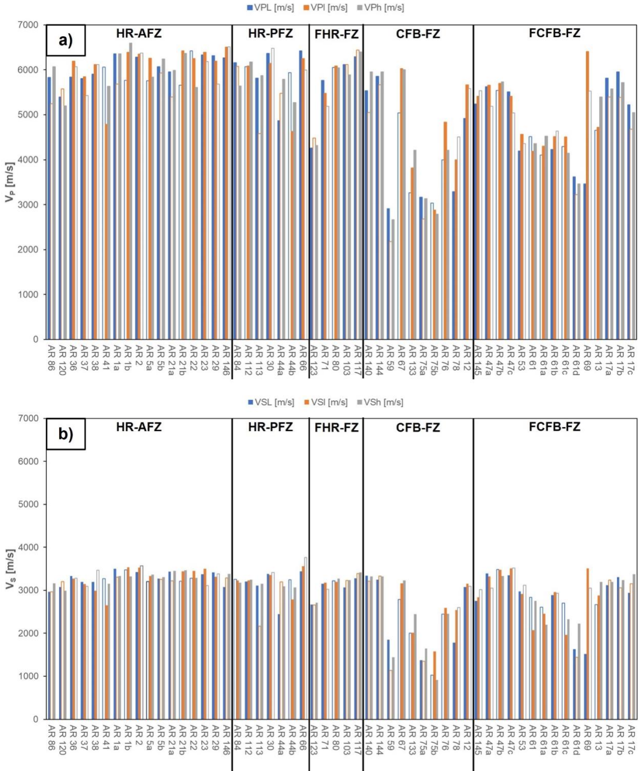
840 Figure A 1: Variation of a) P-wave and b) S-wave velocities evaluated for each sample in each direction. The subscripts L, l, and h refer to the dimensions of the block sample: specifically, L represents the maximum dimension, and h represents the
