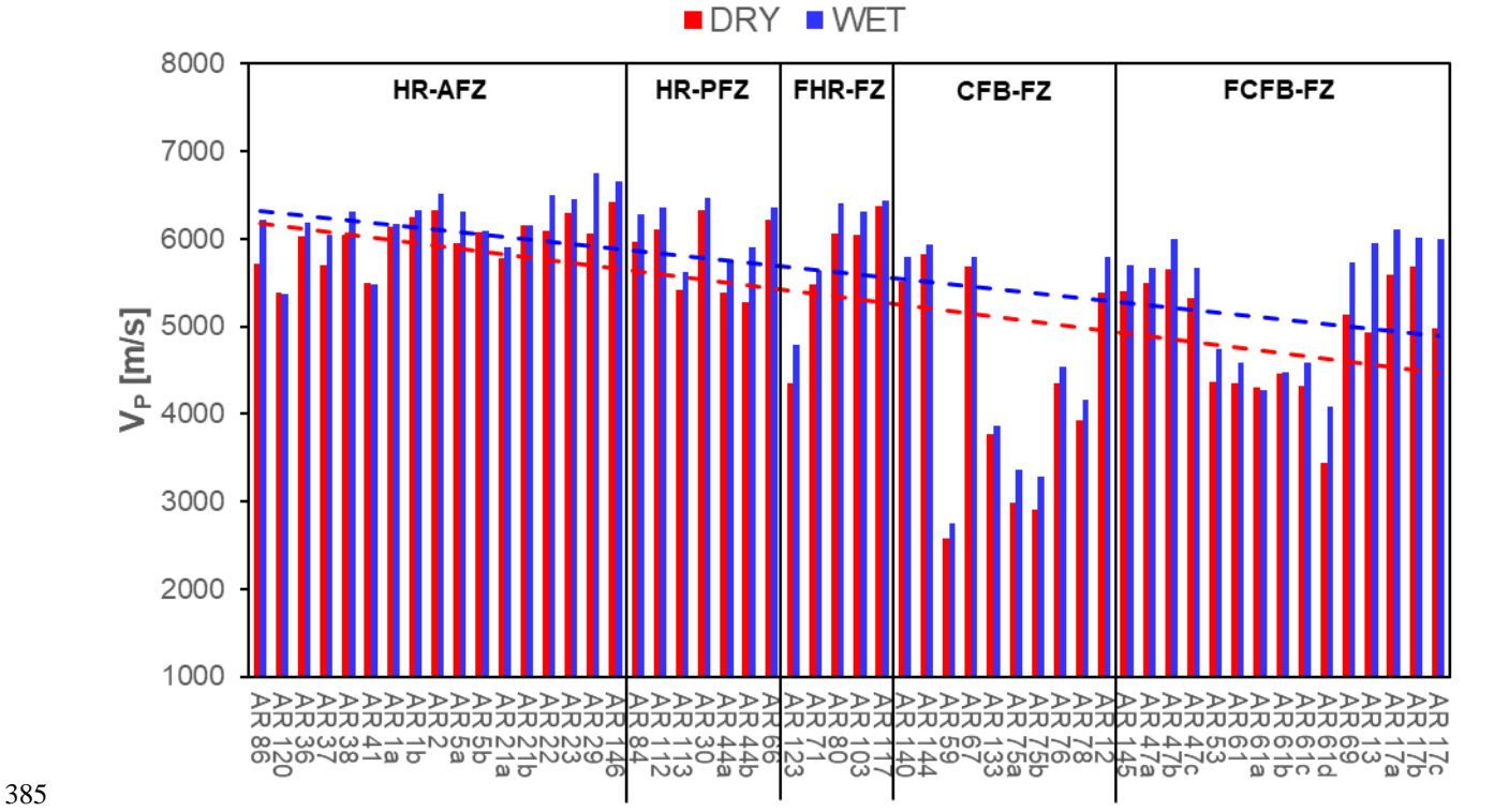
Figure 8: V_P values in dry (red bars) and saturated (blue bars) conditions evaluated as the average of the measurements along the three directions for each rock sample collected in the surrounding of the fault zone.
