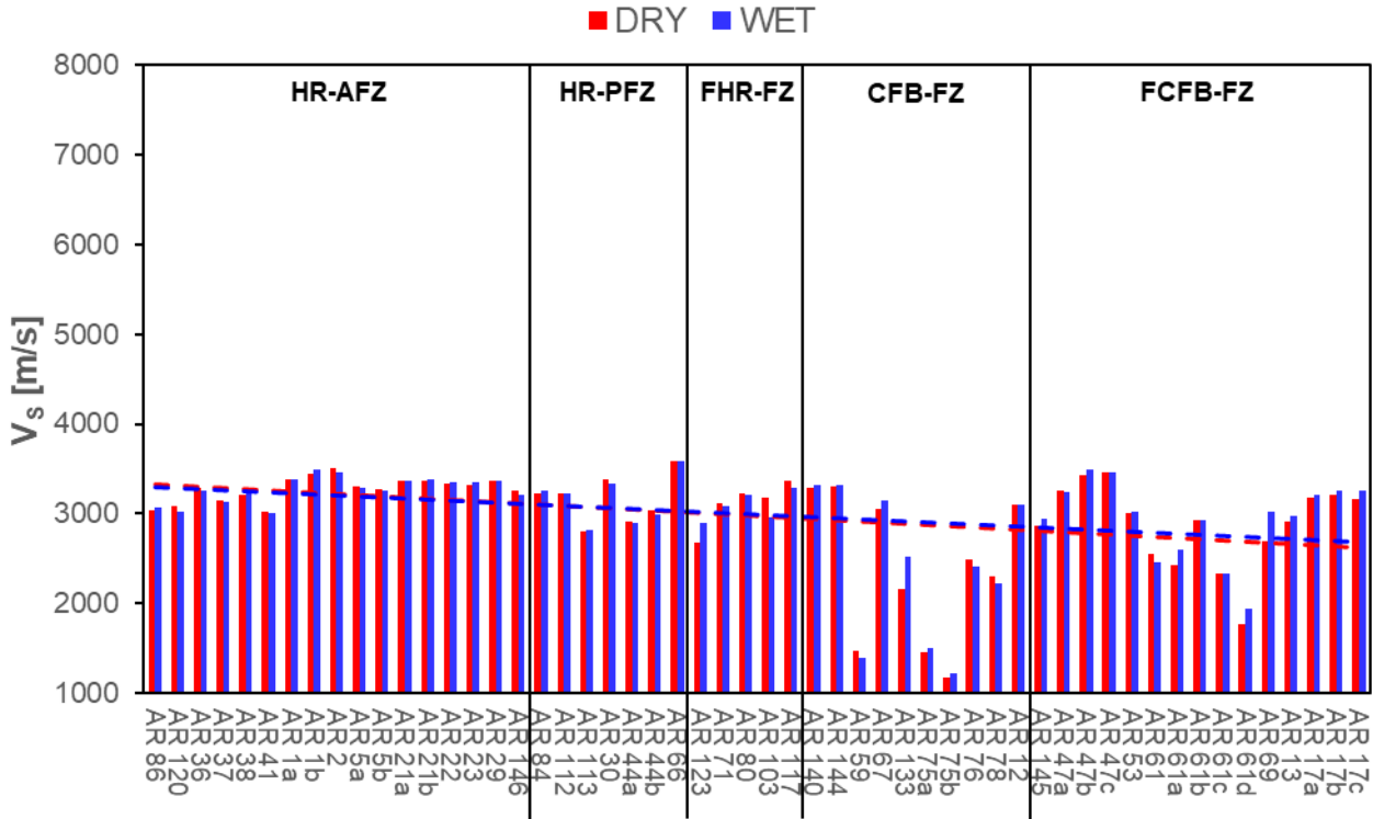
390 Figure 9: V_s values in dry (red bars) and saturated (blue bars) conditions evaluated as the average of the measurements along the three directions for each rock sample collected in the surrounding of the fault zone.
