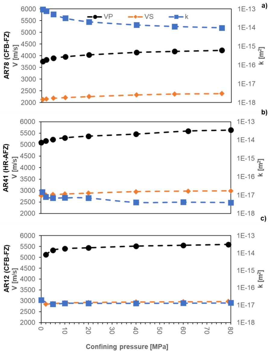
450 Figure 11: Evolution of permeability (blue symbols), V_P (black symbols) and V_S (orange symbols) as a function of confining pressure during gas permeameter tests on sample a) AR78 (CFB-FZ), b) AR41 (HR-AFZ) and c) AR12 (CFB-FZ).
