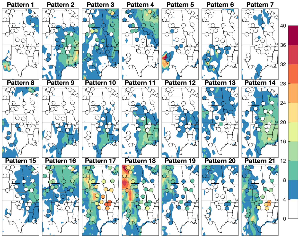
Figure 4. Percentage of each location’s total VIIRS dust counts (background colors) and IMPROVE days that exceed 1\mu\text{g}/\text{m}^3 (points) that occur during each weather pattern. For both VIIRS and IMPROVE data at a particular location, the sum of the panels is 100%.
