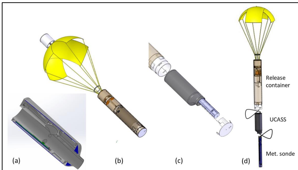
320 Figure 6: (a) Cross-section of OPC UCASS, (b) sonde configuration right after dropping with open parachute, (c) UCASS set free from release container with meteorological sonde (blue) partly within UCASS, and (d) final sonde configuration during measuring flight.
