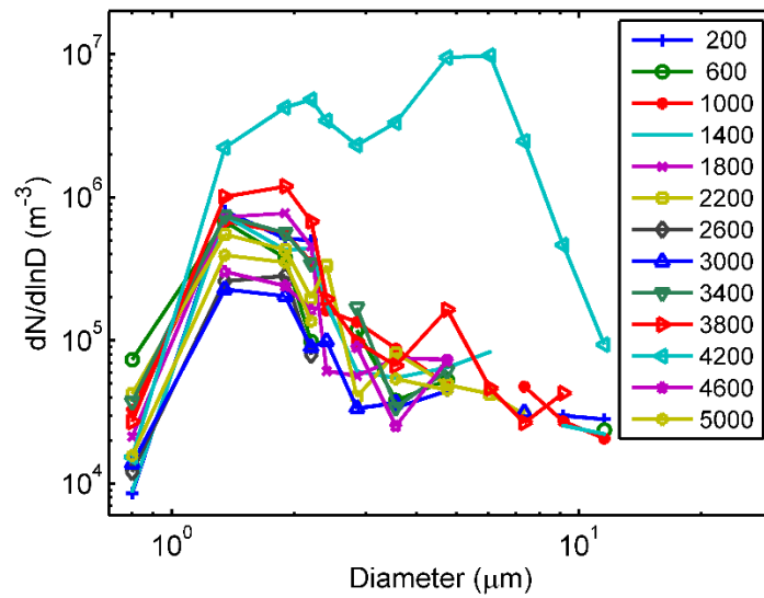
Figure 13: Particle size distributions integrated over 400 m thick layers measured by the sonde U4 during the Saharan dust episode on 03 August. Layer centre altitudes (m) are shown in the legend. The anomalous distribution is due to a thin cloud layer just above 4 km AMSL altitude.
