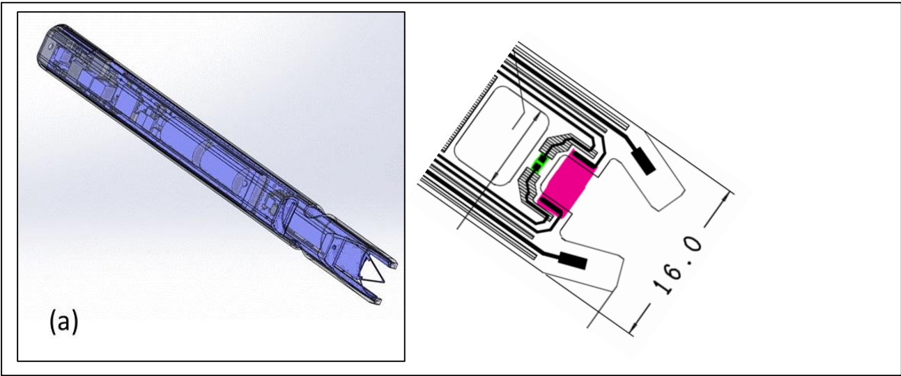
Figure 5: (a) Schematic drawings of the meteorological sonde EL-18 and (b) sensor boom with temperature (magenta) and humidity (green) sensors.
