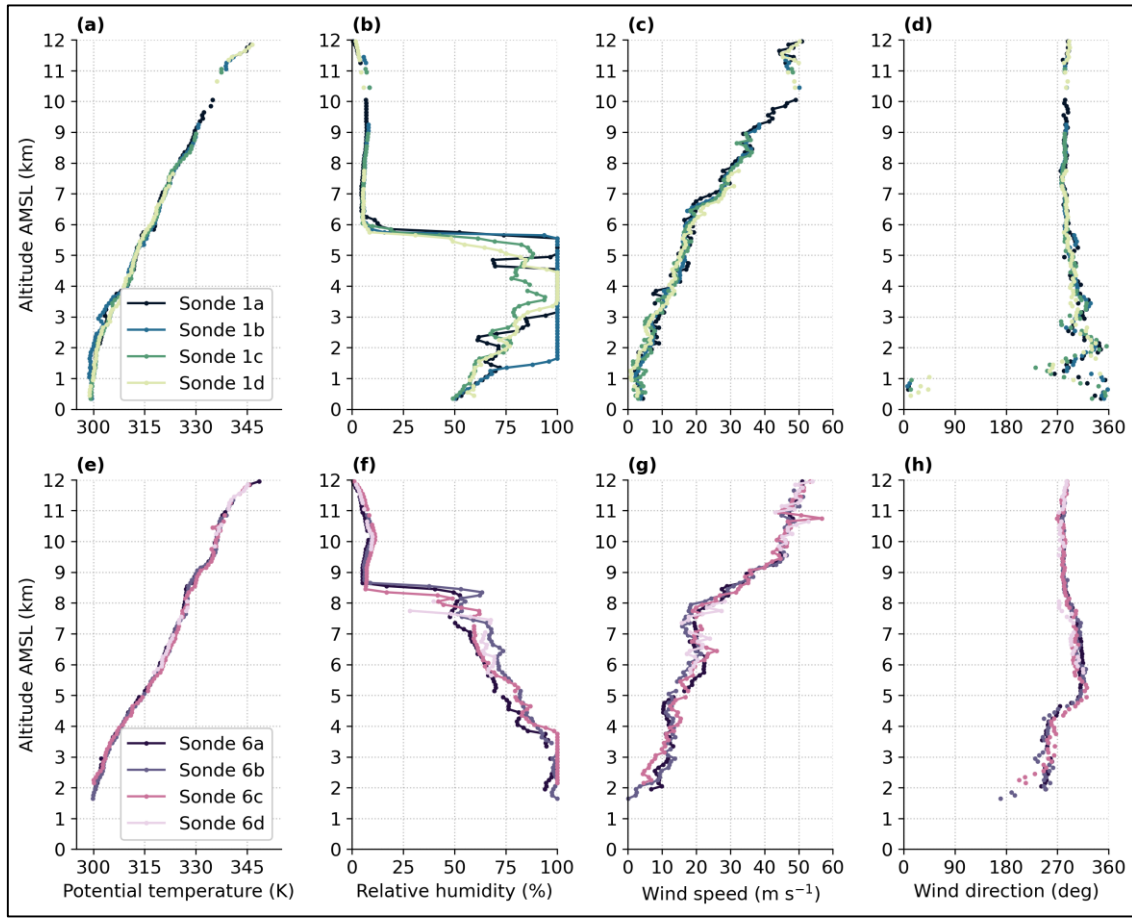
Figure 10: Profiles of (a,e) potential temperature, (b,f) relative humidity, (c,g) wind speed, and (d,h) wind direction of the sondes dropped from the release containers 1 and 6 (see Fig. 8a) on 06 November 2019 at 16:19 and 16:28 UTC, respectively. All profiles are vertically averaged over 100-m intervals.
