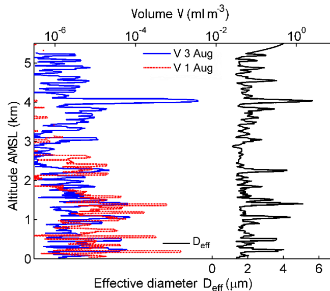
Figure 12: Effective diameter and aerosol volume concentration measured during the Saharan dust episode on 03 August (sonde U4) in comparison with the volume concentration on 01 August (no Saharan dust, sonde U3).
