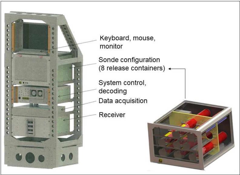
130 Figure 2: KITsonde cabin installation in the aircraft.
