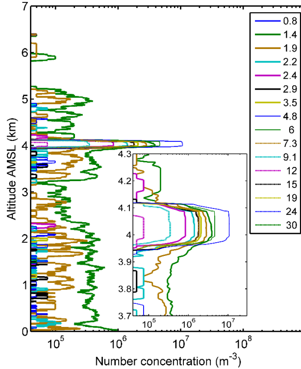
Figure 11: Vertical profile of aerosol concentration during the Saharan dust episode as measured by sonde U4 in 16 size bins, with centre diameter ( \mu\text{m} ) shown in the legend (03 August, 13:13 to 13:33 UTC). Individual concentrations are averaged with a rectangular window width of 20 (i.e. 20 s, equivalent to about 100 m). An embedded shallow cloud layer is visible at 4 km altitude AMSL - inset. See text for further details. Data reprocessed, based on Smith et al. (2019).
