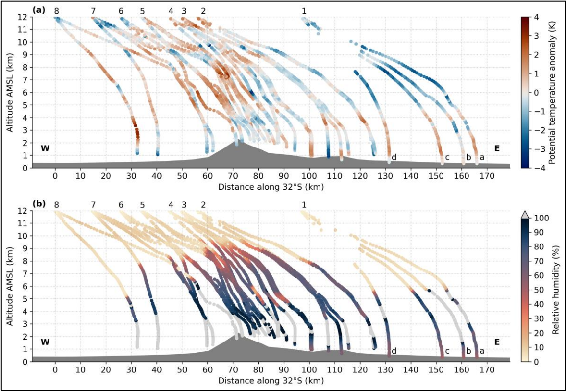
Figure 9: (a) Profiles of potential temperature anomaly (differences from the mean of all shown profiles) and (b) profiles of relative humidity on 06 November of sondes dropped between 16:19 and 16:31 UTC. The numbers at the top of the panel indicate the release containers (corresponding to Fig. 8a). The cloud layers (relative humidity \geq 100 %RH) are shaded in light grey. The distance indicated on the horizontal axis is the projection of the positions of the meteorological sondes onto latitude 32°S. Dark grey shading represents the surface elevation along the transect.
