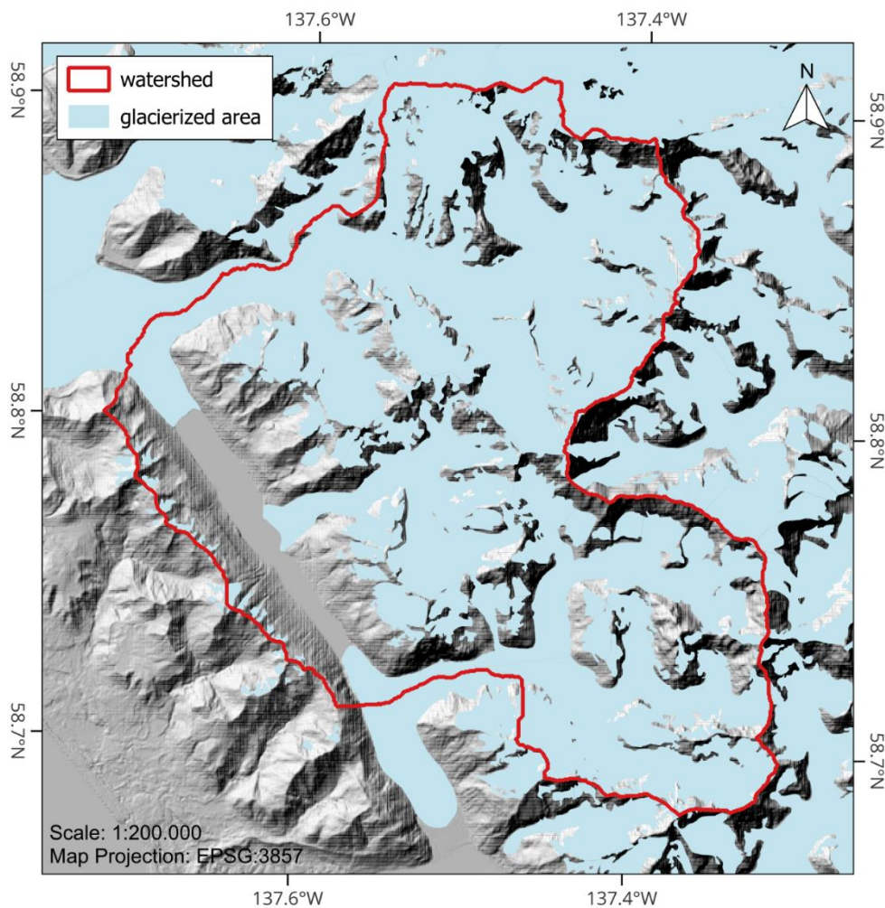
S7: Watershed of Desolation Lake on hill-shaded of the Copernicus DEM (Table S1). Regions highlighted in light blue indicate glacierized areas derived from RGI6.0 (Table S1). The RGI Polygons of Fairweather, Desolation, and Lituya glaciers were clipped at the lake edge to the glacier extents in the DEM.
