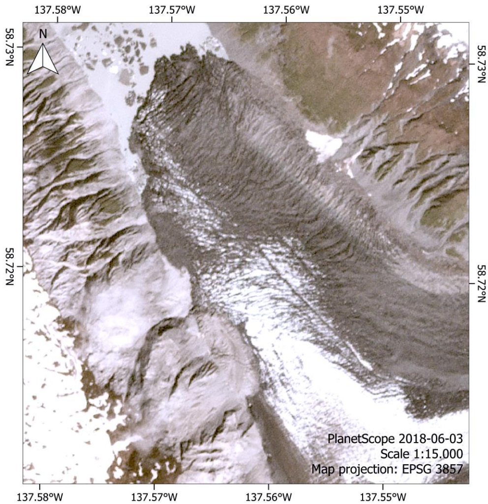
Fig S10: PlanetScope image of the ice dam on 2018-06-03 showing the flow-perpendicular crevasses and detachment of ice at the glacier front towards Desolation Lake.
