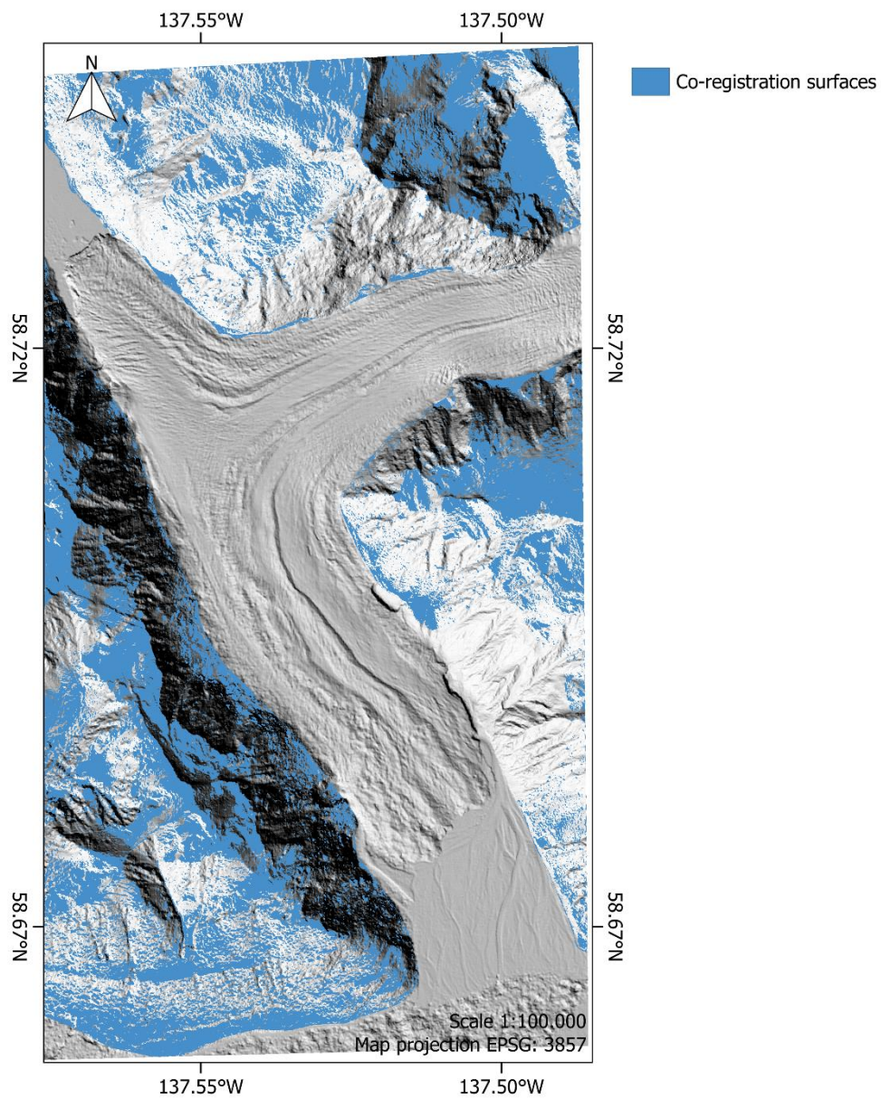
Fig. S3: Map of ArcticDEM co-registration surfaces (blue) draped on a hill-shade of the 2019-04-01 ArcticDEM (Table S1).
