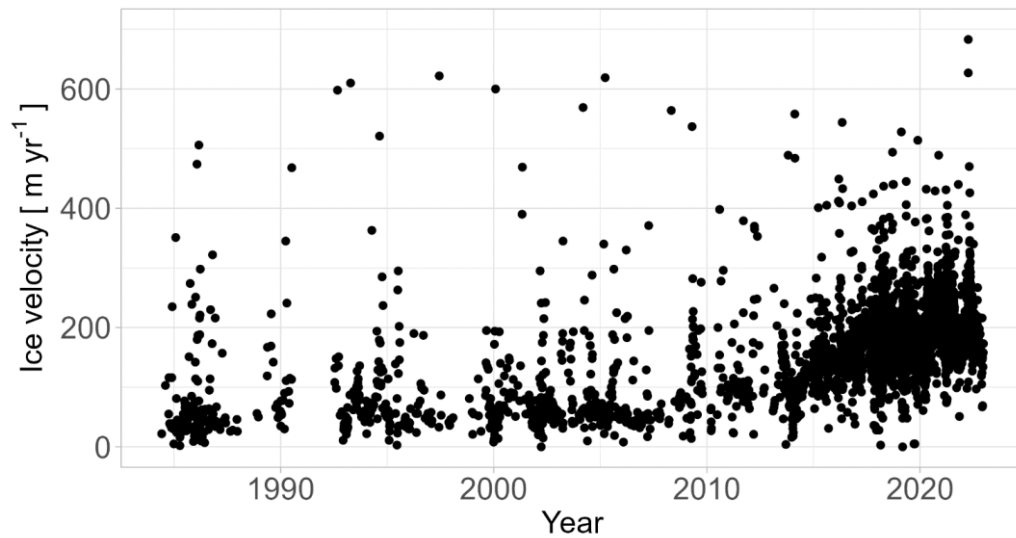
Fig. S8: Ice velocity of Fairweather Glacier at 58.8078^\circ , -137.6848^\circ between 1984 and 2022 extracted from the its_live dataset ( https://its-live.jpl.nasa.gov/ , last access: 2014-06-04). For displaying purposes, six data points with velocities higher than 700 \text{ m yr}^{-1} were excluded in the graph.
