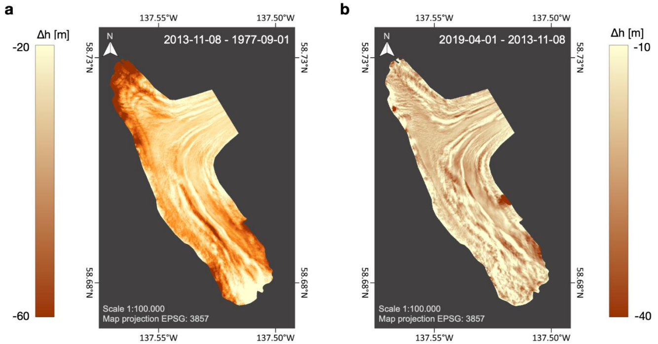
S6: Elevation change across Lituya Glacier dam. a; Vertical point cloud difference between 2013-11-08 and 1977-09-01. b; Arctic DEM difference between 2019-04-01 and 2013-11-08. Note that colormap range differs between the panels.
