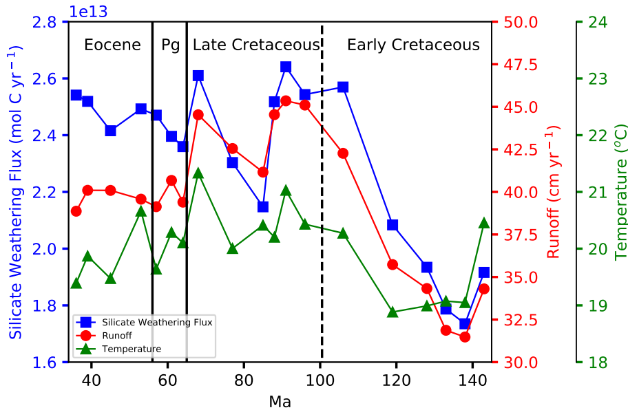
Figure 2. Modelled silicate weathering fluxes (blue squares) plotted against global mean annual runoff (red circles) and temperature (green triangles). Trends in silicate weathering fluxes are similar to those of global runoff, but show less similarity to temperature.
