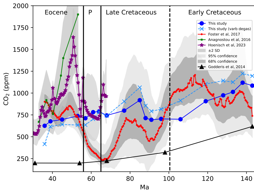
Figure 1. Steady-state CO 2 as modelled by GEOCLIM plotted against two-three CO 2 proxy records from the literature and simulated record from Godd ris et al. (2014). The GEOCLIM model output displays some agreement with the record from Foster et al. (2017), particularly during the early-Cretaceous where CO 2 concentrations are comparably high, the late-Cretaceous, and during the late-Eocene. The CO 2 record from Consortium*† et al. (2023) (referred to here as Hoenisch et al (2023) ) is generally higher than the GEOCLIM model output, but shows a similar pattern in the late Cretaceous and early Palaeocene. The record from Anagnostou et al. (2016) displays considerably higher CO 2 concentrations during the early-Eocene than those in the GEOCLIM and Foster records, but shows better agreement with both records towards the mid and late Eocene. A second GEOCLIM model output (dashed red) displays the results of running GEOCLIM simulations using variable degassing rates calculated in Van Der Meer et al. (2014). Note: Palaeocene is abbreviated to P for brevity.
