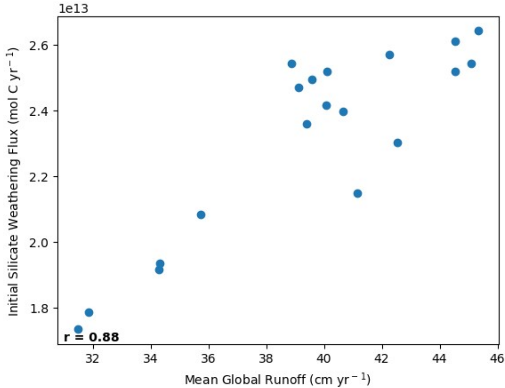
Figure A2. Scatter plot of mean global runoff ( \text{cm yr}^{-1} ) and initial silicate weathering fluxes from the earliest-Cretaceous (s) to the latest-Eocene (A) 19 modelled timeslices. Zonal-Global runoff means are low in the early-Cretaceous and silicate weathering fluxes show a strong positive correlation ( s\text{-p}R = 0.88 ), but increase significantly into the mid-Cretaceous, especially in the northern mid-latitudes (o-k). Zonal mean runoff falls slightly into the late-Cretaceous, but there is an intensification in equatorial mean zonal runoff (j-h). In the Cenozoic, zonal runoff intensifies again (g-e) but begins to weaken again during the Eocene (d-a).
