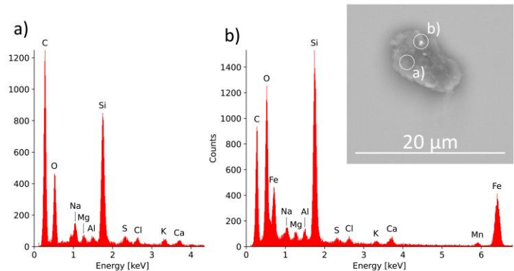
445 Figure 7: EDX spectra and BSE image of a C-rich INP (a) with Fe-rich areas (b).
