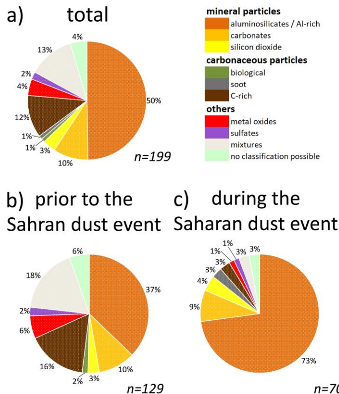
585 Figure 11: Chemical INP composition with the number of analyzed particles (n) from CLACE/INUIT 2017 at the high-altitude research station Jungfraujoch (activated at T = -30 °C and RH = 99 / 101 %; RH = 95 / 97 % was chosen for one sample due to cluster formation at higher RH). a) total composition over the whole campaign period; b) composition prior to the Saharan dust event and c) during the Saharan dust event. For confidence intervals see supplement Tab. S1.
