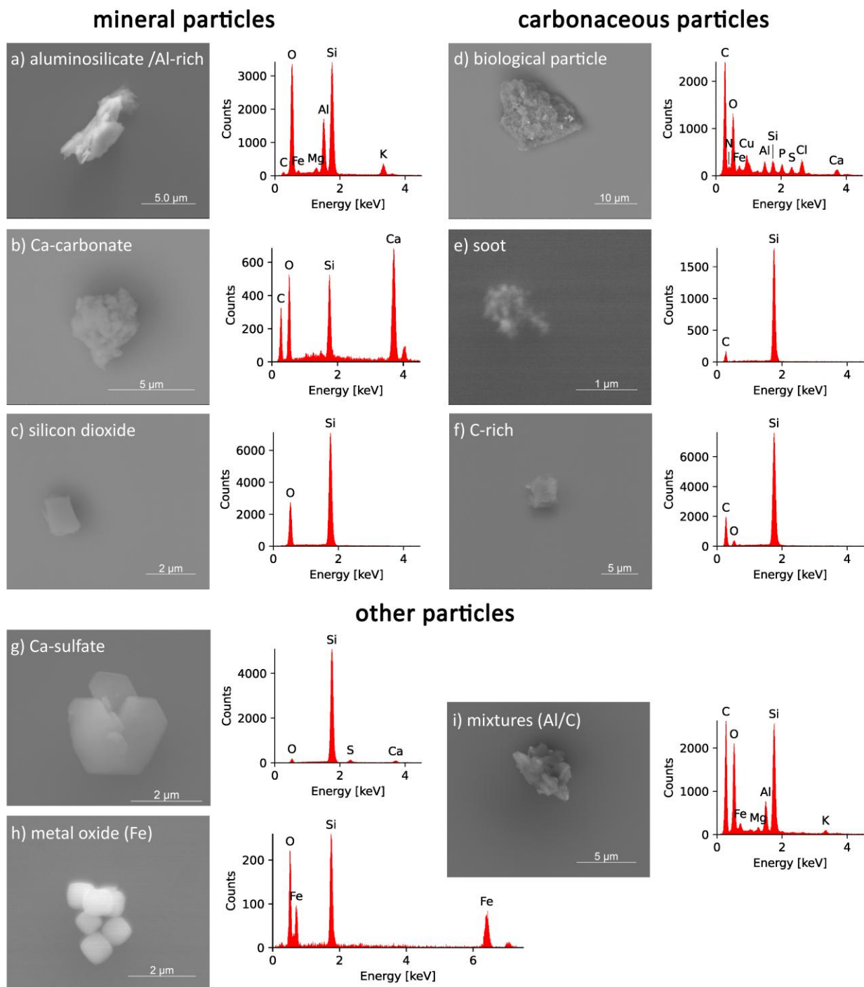
530 Figure 10: Overview of representative EDX spectra and corresponding SEM images for the defined INP classes grouped as mineral particles (aluminosilicate / Al-rich (a), Ca-carbonate (b), silicon dioxide (c)), carbonaceous particles (biological particles (d), soot (e), C-rich (f)) and other particle classes (Ca-sulfate (g), metal oxide (h), mixtures (i)).
