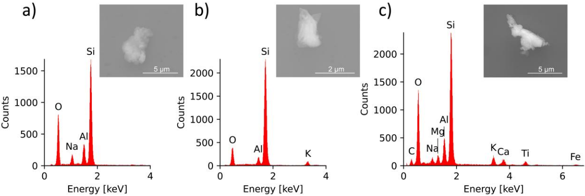
490 Figure 9: EDX spectra and SE-images of various aluminosilicates: a) Na-containing aluminosilicate; b) K-containing aluminosilicate; c) complex aluminosilicate
