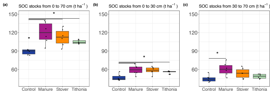
370 Figure 2: Total stocks of organic carbon for (a) the 0-70 cm soil layer, (b) the topsoil (0-30 cm) and (c) the subsoil (30-70 375 cm). Significant difference between organic residues treatments and control are highlighted with a “*”.
