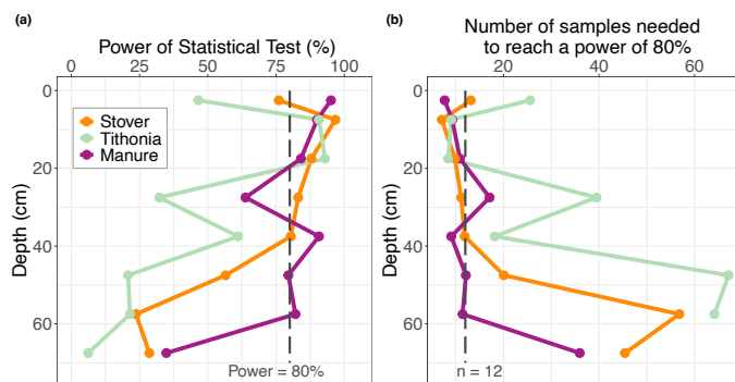
420 Figure 4: (a) Power of statistical analysis at each depth layer and for each organic residue treatment and at each 5 cm 425 depth layer. The 80% power threshold is indicated by the dashed line. (b) The amount of sample samples required to reach a statistical power of 80% for each organic residue treatment and each 5 cm depth layer. The actual number of sample ( n = 12) is indicated by the dashed line.
