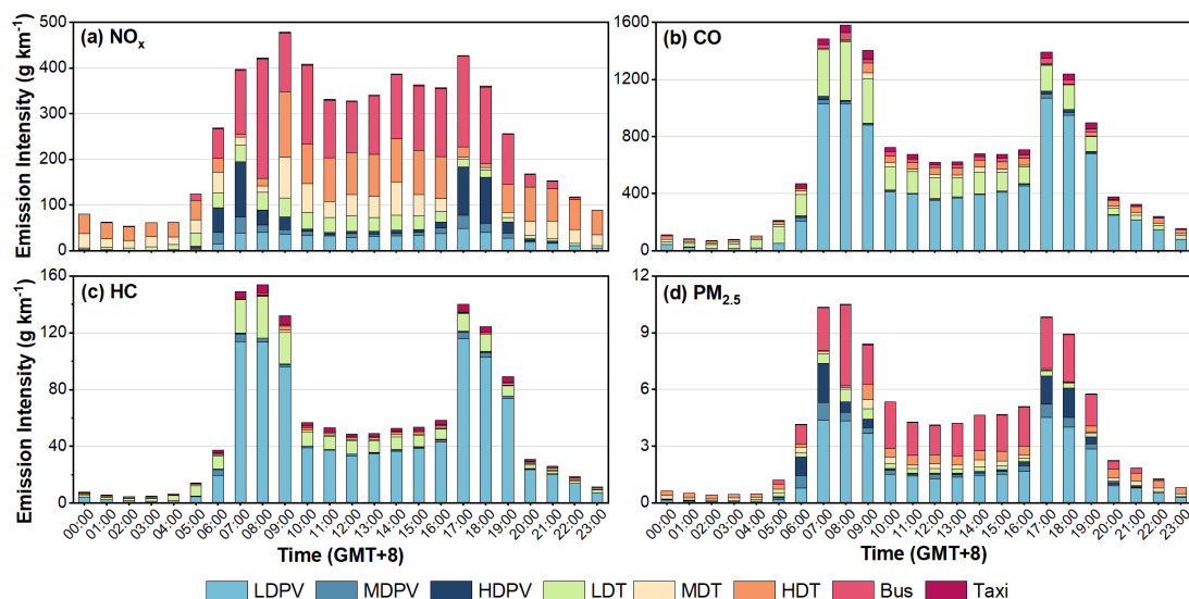
335 Figure 4. Average hourly emission intensities from different types of vehicles at traffic monitoring points for (a) NO x , (b) CO, (c) HC, and 340 (d) PM 2.5 .
