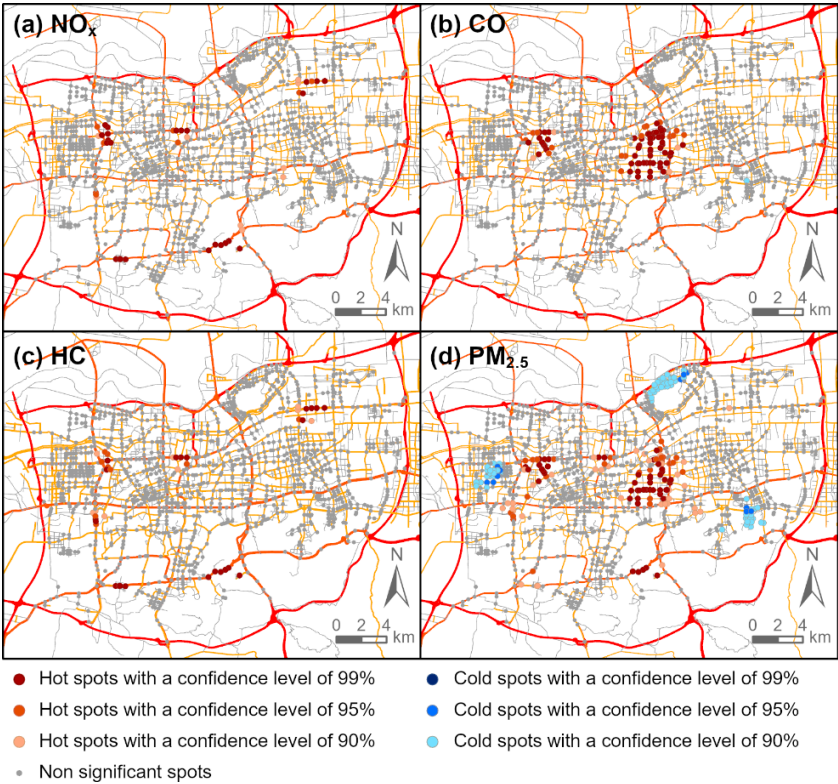
465 Figure 9. Spatial distributions of hot and cold spots of on-road vehicle emissions for (a) NO x , (b) CO, (c) HC, and (d) PM 2.5 .
