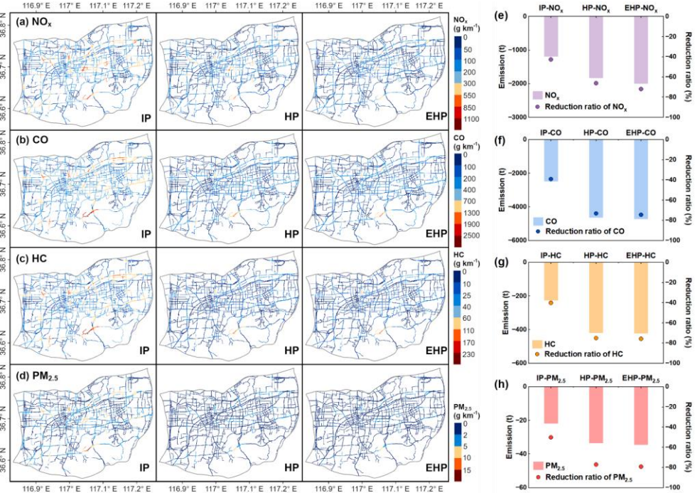
Figure 10. On-road vehicle emission mappings for (a) NO x , (b) CO, (c) HC, and (d) PM 2.5 simulated under different new energy penetration scenarios and emission reductions for (e) NO x , (f) CO, (g) HC, and (h) PM 2.5 under each scenario relative to the base case during the study period. Bars indicate the emission reduction amounts and dots indicate the percentage reduction.
