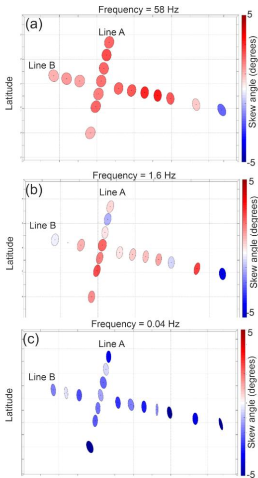
330 Figure 8. Phase tensor at frequencies of 58 Hz, 1.6 Hz and 0.04 Hz plotted in map view. The direction of the major and minor axes of the ellipses show to possible strike directions. Circles indicate a 1D structure while ellipses indicate a 2D or 3D structure. This direction variation varies with frequency but is consistent with the direction of the trough axis which is N105E. The colour fill shows the skew angle of (Caldwell et al., 2004). Values close to zero indicate a 1D or 2D resistivity structure. Non-zero values indicate a 3D resistivity structure.
