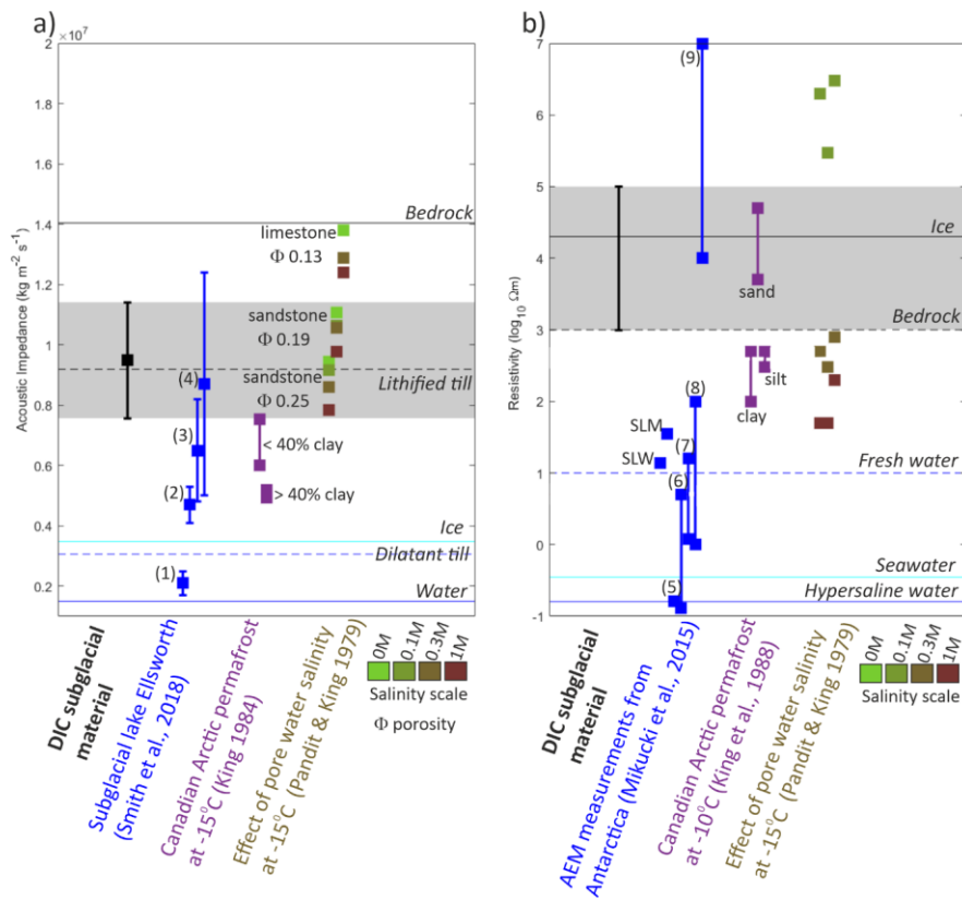
365 Figure 10. Properties of the material in the trough directly beneath DIC. a) Acoustic impedance compared to that of subglacial material from subglacial lake Ellsworth: 1) lakebed, subaqueous, soft wet sediment, (2) subglacial, soft wet sediments, (3) hard bed, wet sediments and (4) hardest bed, rock or frozen sediment (Smith et al., 2018), and laboratory studies measuring the acoustic properties of permafrost and sedimentary samples collect in the Canadian Arctic at -15°C (King, 1984; Pandit & King, 1979). Horizontal coloured lines represent estimated acoustic impedance values for different materials detailed in Peters et al. (2008). b) Resistivity compared to that of subglacial lake Whillans (SWL; Christner et al., 2014) and Mercer (SLM; Priscu et al., 2021) direct samples, airborne electromagnetic (AEM) measurements from the Taylor Dry Valleys, Antarctica ((5) Blood Falls outflow, (6) west lake Bonney between 5 m and 35 m depth, (7) lake Fryxell between 5 m and 18 m depth, (8) sediments with brine in the pores and (9) glacier ice (Mikucki et al., 2015), and laboratory studies measuring the resistivity of permafrost and sedimentary samples collect in the Canadian Arctic at temperature <-10°C (Pandit & King, 1979; King et al., 1988). Horizontal coloured lines represent estimated resistivity values for different materials detailed in Killingbeck et al., (2021) and Key and Siegfried (2017). 370
