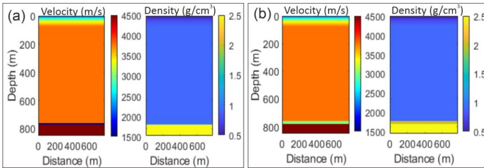
495 Figure A1. (a) V_p and density model used to compute the synthetic model shown in C. (b) V_p and density model used to compute the synthetic model shown in D. (c) Devon shot gather compared with synthetic seismic data for a 10 m thick subglacial lake, with a zoomed in window of the reflected wavelets.
