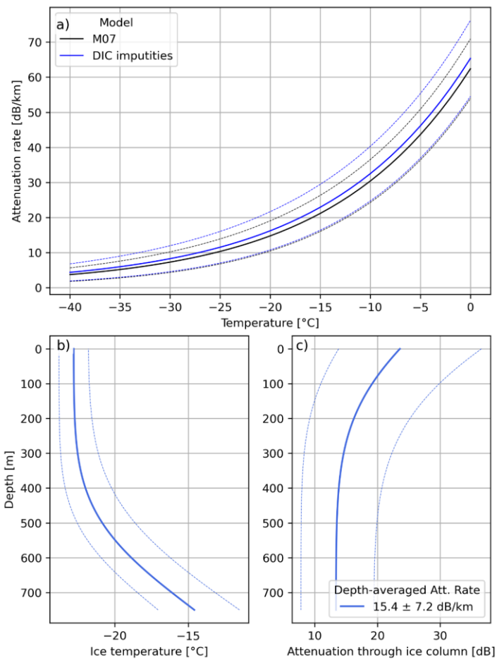
520 Figure D1. (a) Attenuation rate as a function of ice temperature from the models used over DIC and Greenland (M07). (b) Example ice temperature profiles including their uncertainty ranges, and (c) resulting attenuation rates (one-way) through the ice column, propagating ice temperature and impurity uncertainties.
