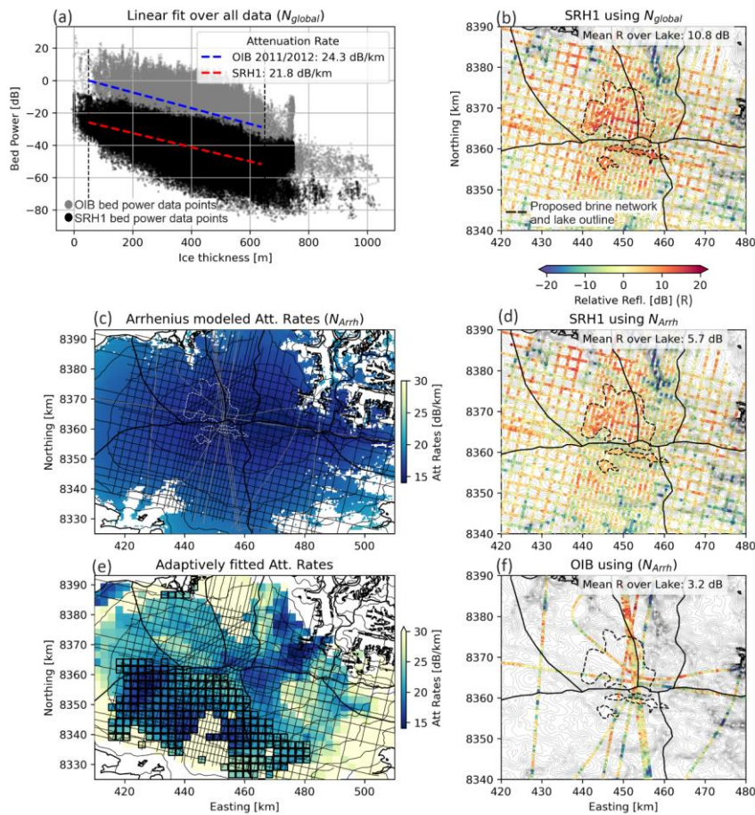
430 Figure 11. Re-analysis of radar attenuation rates and reflectivity over DIC. (a) Linear regression fits (over entire DIC datasets) to 435 derive attenuation rates ( N_{global} ) from the Operation Ice Bridge (OIB) MCoRDS radar data (2011, 2012) used in (Rutishauser et al., 2018) (grey) and the SRH1 HiCARS data used in (Rutishauser et al., 2022) (black). (b) SRH1 basal reflectivity (Rutishauser et al., 2022) corrected using a constant ( N_{global} ) rate of 21.8 dB/km (linear regression in a). (c) Arrhenius modeled attenuation rates over DIC. Black and grey thin lines are the SRH1 and OIB 2011/2012 survey lines, respectively. (d) SRH1 basal reflectivity corrected using the Arrhenius modelled attenuation rates ( N_{Arrh} , shown in c). (e) Attenuation rates derived from the SRH1 dataset via an adaptive fitting approach (Schroeder et al., 2016; Chu et al., 2021). Black squares indicate areas where the minimum fit criteria are not met (Appendix D). (f) OIB 2011/2012 basal reflectivity corrected using the Arrhenius modelled attenuation rates (shown in c). All attenuation rates are noted as one-way attenuation rates.
