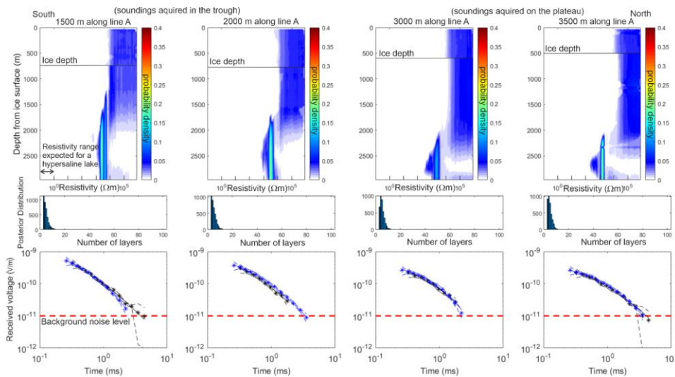
290 Figure 6. Line A TEM Bayesian inversion results for the 7.5 Hz and 3 Hz base frequencies. Top plot: posterior distribution of resistivity with depth. Middle plot: posterior distribution of the number of layers. Bottom plot: comparison of data fit plot, with the best fitting forward model accepted in the ensemble (-) compared to the data (*) and error tolerance (-). The black data points are the 3 Hz base frequency, and the blue data points are the 7.5 Hz base frequency. The red dashed line is the background noise level.
