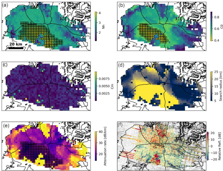
455 Figure 12. Results and correlation-fit parameters from the adaptive attenuation fitting approach (Schroeder et al., 2016; Chu et al., 2021). (a) Half-width of the correlation coefficient minimum N_h . (b) Uncorrected correlation coefficient magnitude C_0 . (c) Minimum correlation coefficient C_m . (d) Search radius used to derive the resulting attenuation rate (either criteria are met, or maximum search radius of 25 km is reached). (e) One-way attenuation rate. Black squares mark areas where the minimum fit criteria of N_h \leq 3 dB/km (a) or C_0 \geq 0.5 (b) are not met. (f) Relative basal reflectivity upon application of the attenuation rates in (e). 460
