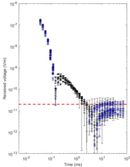
500 Figure B1. Raw TEM data for all soundings with error bars. Blue circles are negative received voltages and back dots are positive received voltages. The red line indicates the estimated background noise level.
