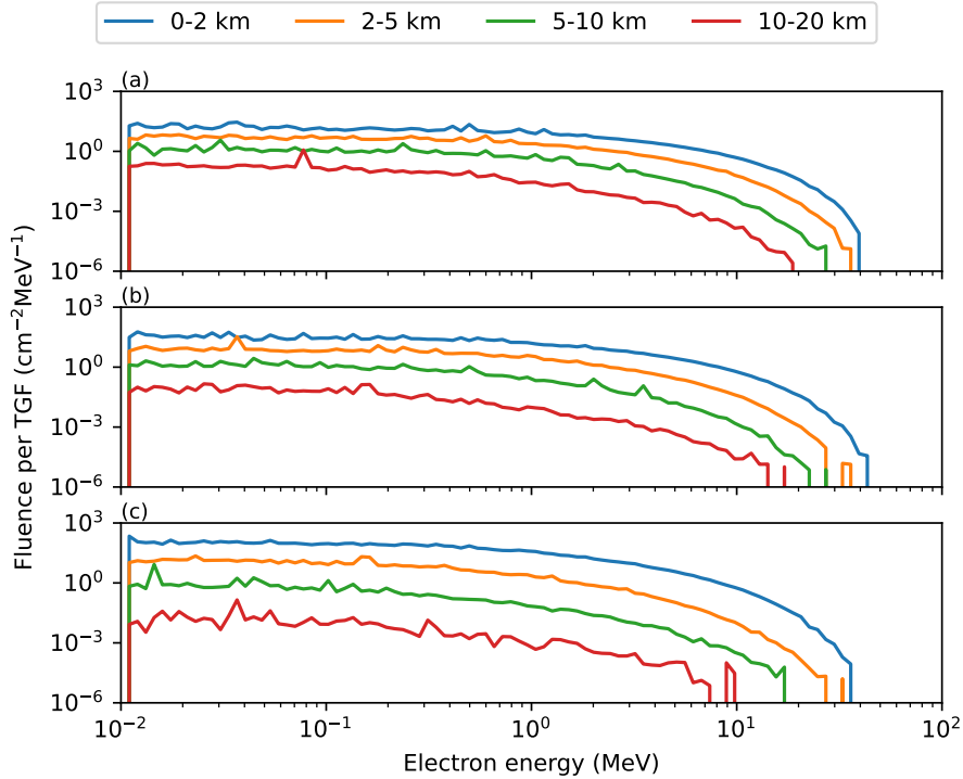
Figure 9. Energy spectra of electrons caused by a TGF for different radial distances from the TGF origin. The altitude of the TGF origin is 15 km, and energy spectra are recovered from altitudes of a) 30 km, b) 25 km, c) 20 km.
