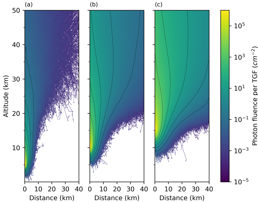
Figure 2. Fluence of photons caused by a TGF at an altitude of a) 5 km, b) 10 km, c) 15 km. The depicted isobars show photon fluences of 10^0 , 10^1 , 10^2 , 10^3 \text{cm}^{-2} .
