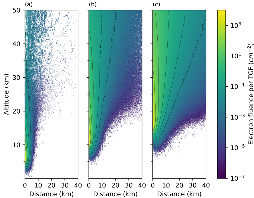
Figure 7. Fluence of electrons caused by a TGF at an altitude of a) 5 km, b) 10 km, c) 15 km. The depicted isobars show electron fluences of 10^{-2} , 10^{-1} , 10^0 , 10^1 , 10^2 \text{cm}^{-2} .
