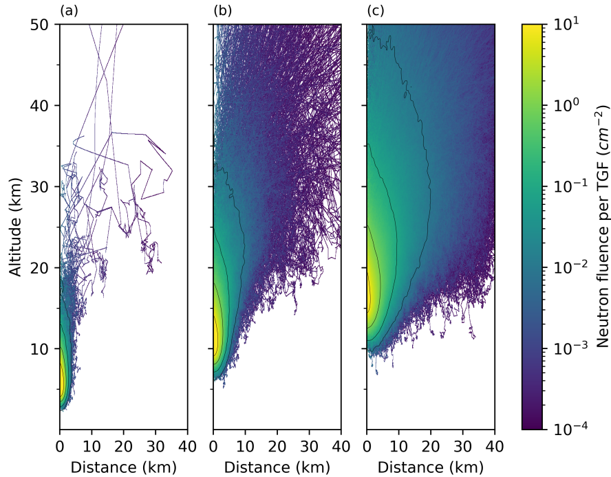
Figure 11. Fluence of neutrons caused by a TGF at an altitude of A) 5 km, B) 10 km, C) 15 km. The depicted isobars show neutron fluences of 10^{-2} , 10^{-1} , 10^0 , 10^1 \text{cm}^{-2} .
