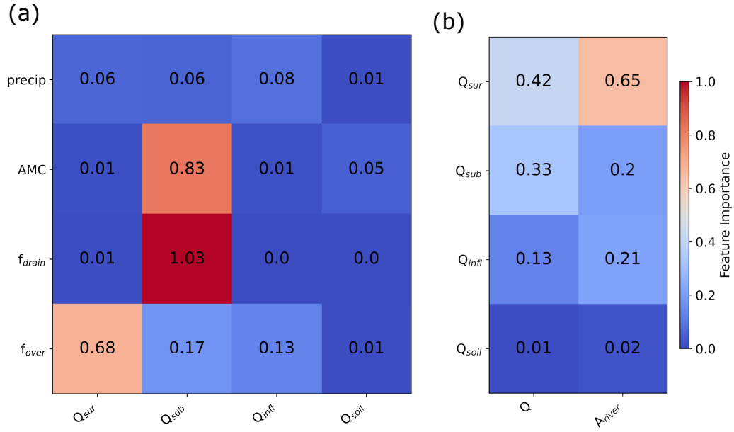
445 Figure 9: (a) Permutation importance of perturbation parameters (precipitation, AMC, f_{drain} and f_{over} ) on hydrological drivers of Q_{sur} , Q_{sub} , Q_{infl} and Q_{soil} . The corresponding box plot of each driver is provided in row 1~4 of Figure S8. (b) Permutation importance of hydrological drivers on river discharge ( Q ) and flooded area ( A_{river} ). The coastal inundation area ( A_{ocean} ) is not considered from this analysis as MPAS-O is excluded from the expanded ensemble simulations. The scatter plots of Q and A_{river} against the drivers are respectively provided in the 5th and 6th rows of Figure S6.
