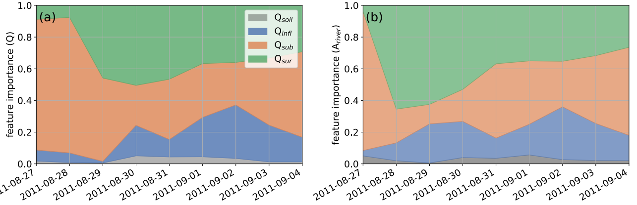
450 Figure 10: Time evolution of permutation importance (scaled between 0 and 1) of the four hydrological drivers for (a) Q and (b) A_{river} . The corresponding skill scores ( r^2 and NRMSE) of the ANNs trained using daily data are provided in Figure S9. The Irene-induced peak river discharge is on August 30, 2011.
