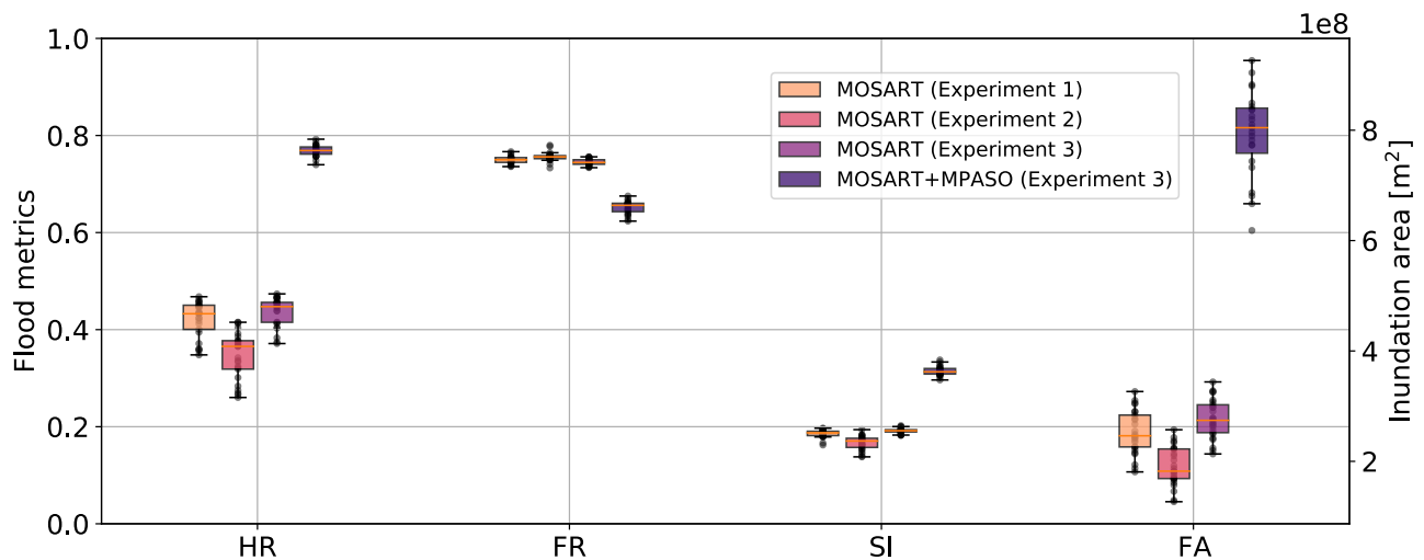
Figure 5: Flood metrics of hit rate ( HR ), false rate ( FR ), success index ( SI ) and flooded area ( FA ) used to compare riverine flooding in Experiments 1~3 and the combined riverine and coastal flooding in Experiment 3. Experiment 1 and 2 include land and river components, while Experiment 3 runs all land, river and ocean components (Table 1). MOSART only considers riverine
