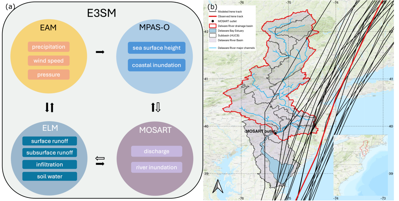
Figure 2: (a) The multi-component E3SM framework and drivers used for analyses within each model component. The black arrows represent the data flow via the one-way coupled framework. The white arrows are the new flow directions from the 2-way land-river and river-ocean models. (b) Map of Delaware river basin (DRB), Delaware bay estuary (DBE), and the observed (red) and modeled (black) Irene tracks. The topographic map in (b) is from the ESRI world topographic map (ESRI, 2012).
