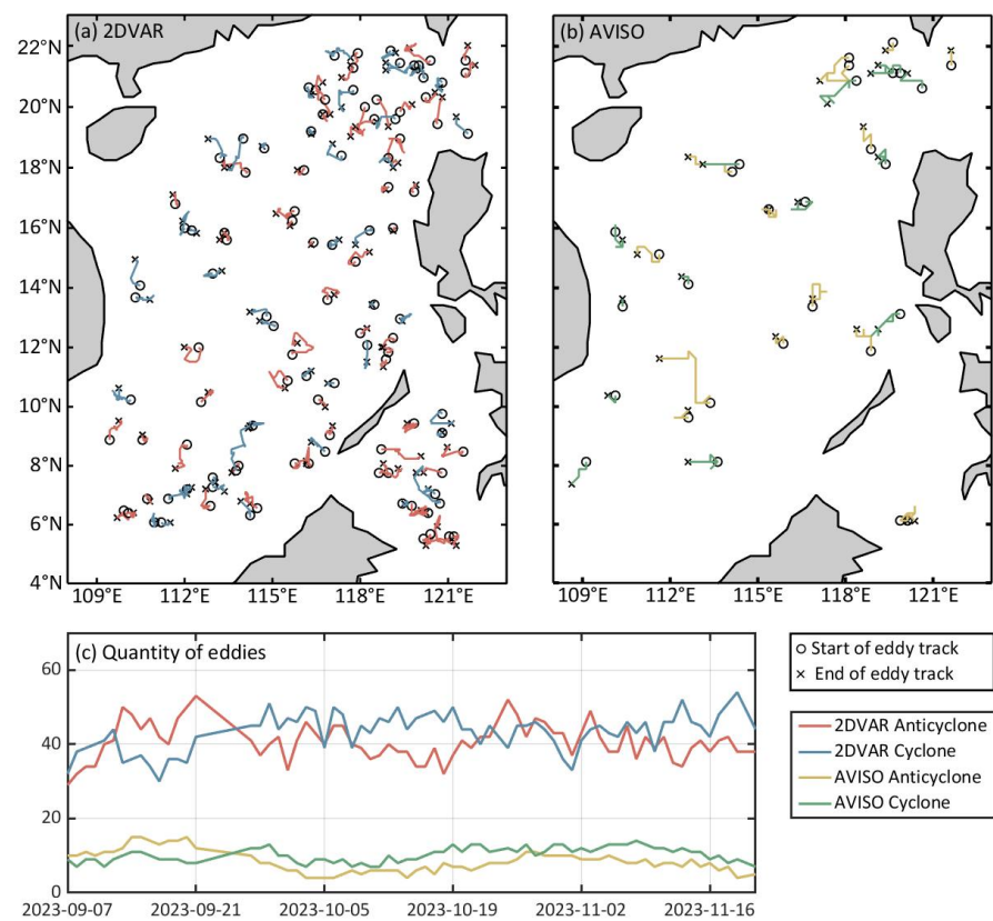
Figure 6. Eddies and tracks identified during the SWOT science phase (cycle number from 3 to 6, time period from 2023/09/06 to 11/21) in (a) 2DVAR and (b) AVISO merged maps. The red (yellow) and blue (green) lines represent the anticyclone and cyclone tracks in the 2DVAR (AVISO) merged maps, respectively. The black circles and crosses indicate the start and end positions of the eddies, respectively. (c) The number of eddies over time. The red (yellow) and blue (green) lines represent the daily count of anticyclones and cyclones, respectively, as identified in the 2DVAR (AVISO) merged maps.
