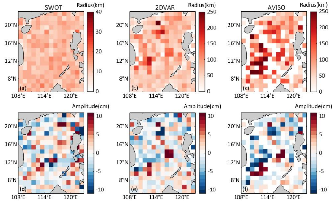
Figure 7. Distributions of eddy radius (top) and amplitude (bottom) for SWOT (left column), 2DVAR (middle column), and AVISO (right column) from 2023/09/06 to 11/21 are presented. The colour intensity is proportional to the radius, with darker colours indicating larger radii. Similarly, the colour intensity is proportional to the amplitude, with darker red (blue) indicating larger positive (negative) amplitudes.
