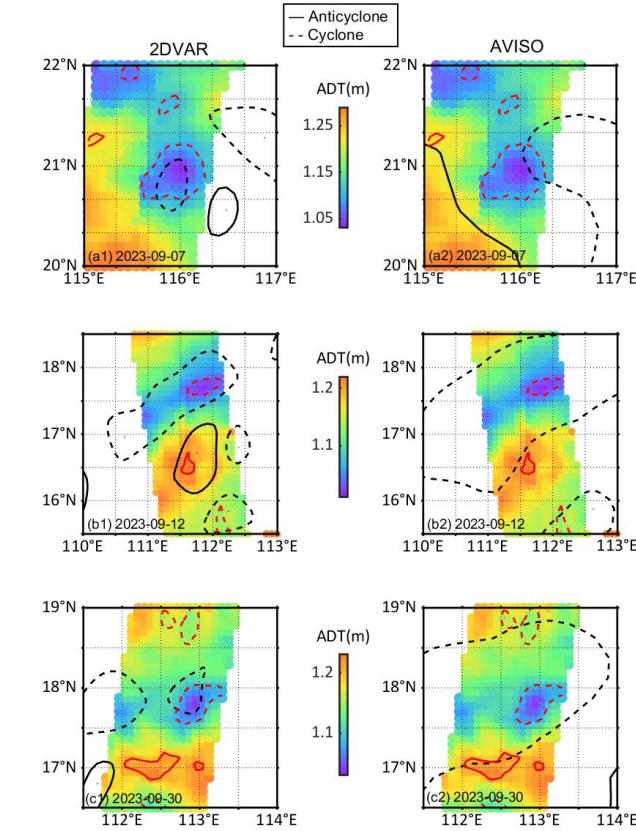
Figure 3. The ADT observation data of SWOT with the eddies detected by SWOT (in red), 2DVAR (in black, a1-c1) and AVISO (in black, a2-c2). The solid line represents the anticyclonic eddies and dashed line represents the cyclonic eddies.
