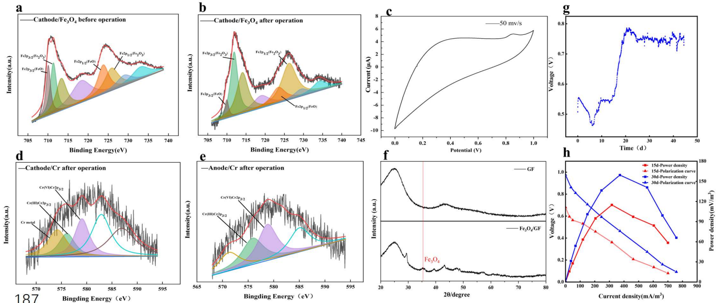
188 Fig. 2 Characterization of electrode materials and power generation performance of 189 SMFC. (a-b) Fe2p spectra of cathode/Fe 3 O 4 composite cathode, (c) cyclic voltammetry 190 (CV) curve of cathode/Fe 3 O 4 , (d-e) Cr2p spectra of GF composite cathode and Anodic 191 Aluminum foam after operation, (f) XRD spectrum of the cathode-Fe 3 O 4 ; (g) SMFC 192 output voltage distribution, (h) 15-day vs. 30-day polarization curves and power density 193 curves of the SMFC.
