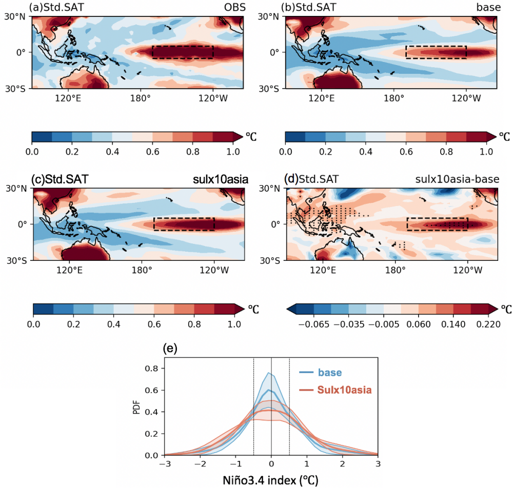
Figure 3. DJF multimodel mean standard deviations of SAT (SST over the ocean, °C) from (a) observations during 1965-2014, (b) coupled baseline simulations, (c) coupled SUL×10Asia simulations. (d) Differences in standard deviations of SAT (SST over the ocean, °C) between coupled SUL×10Asia and baseline simulations. Dotted regions indicate significant differences at the 95% level from the two-tailed F -test. (e) Frequency distributions of the Niño3.4 index from coupled simulations in PDRMIP with multimodel-means (thick coloured curves) and the associated 95% confidence intervals (coloured shades). The confidence intervals are estimated from different models by using bootstrap resampling.
