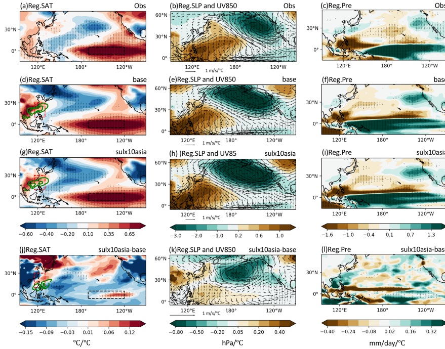
Figure 1. DJF regressions of (a)(d)(g), surface air temperature (SAT, SST over the ocean, °C, shading) and 1000 hPa meridional wind (V1000) over the broad East Asia (green contours, values plotted only when larger than 0.1 m s -1 °C -1 ), (b)(e)(h) sea level pressure (SLP; hPa, shading) and 850 hPa wind (UV850; m s -1 , vector), (c)(f)(i) precipitation (Pre, mm d -1 ) onto the Niño3.4 index from (a-c) observations during 1965-2014, multimodel mean coupled (d-f) baseline and (g-i) SUL×10Asia simulations in PDRMIP. Dotted regions indicate significant correlations at the 95% level from the two-tailed Student's t test. Differences in regressions of (j) SAT and V1000 (green contours, values plotted only when larger than 0.05 m s -1 °C -1 ), (k) SLP and UV850, (l) Pre between coupled SUL×10Asia and baseline simulations. Dotted regions represent differences that remain significant after false discovery rate (FDR) correction of p -values from two-tailed Student's t -test (Wilks et al., 2016). The definition regions of the EAWM index and the Niño3.4 index are marked by red and black rectangles respectively.
