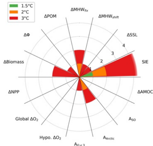
Figure 6: Same as Figure 5, but according to global warming levels (1.5°C, 2°C and 3°C) under the SSP5-8.5 scenario. Therefore, ASAT is not shown.
