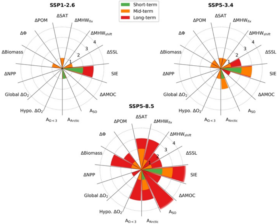
Figure 5: Exceedance of mitigation limits with high probability ( >80\% of the CMIP6 models) in the near-term (2021-2040), mid-term (2041-2060) and long-term (2081-2100) periods under (left) SSP1-2.6, (right) SSP5-3.4-OS and (middle) SSP5-8.5 scenarios.
