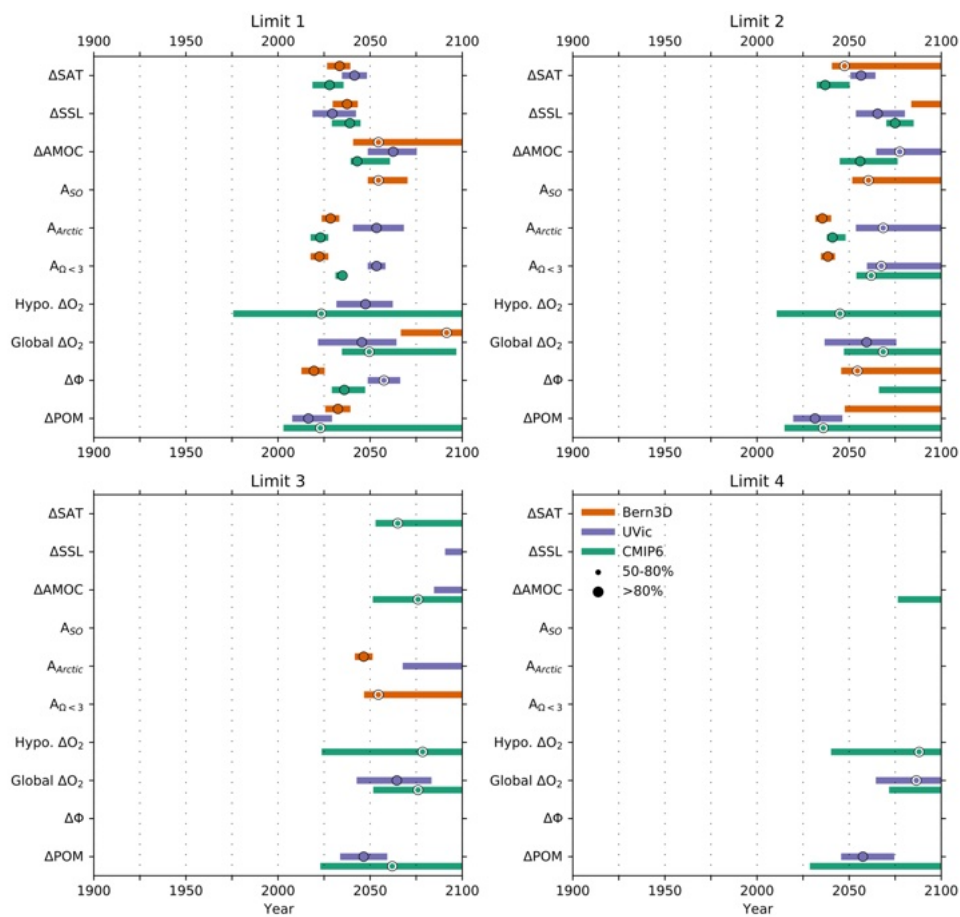
965 Figure A4: Same as in Figure 7 but for SSP5-3.4-OS.
