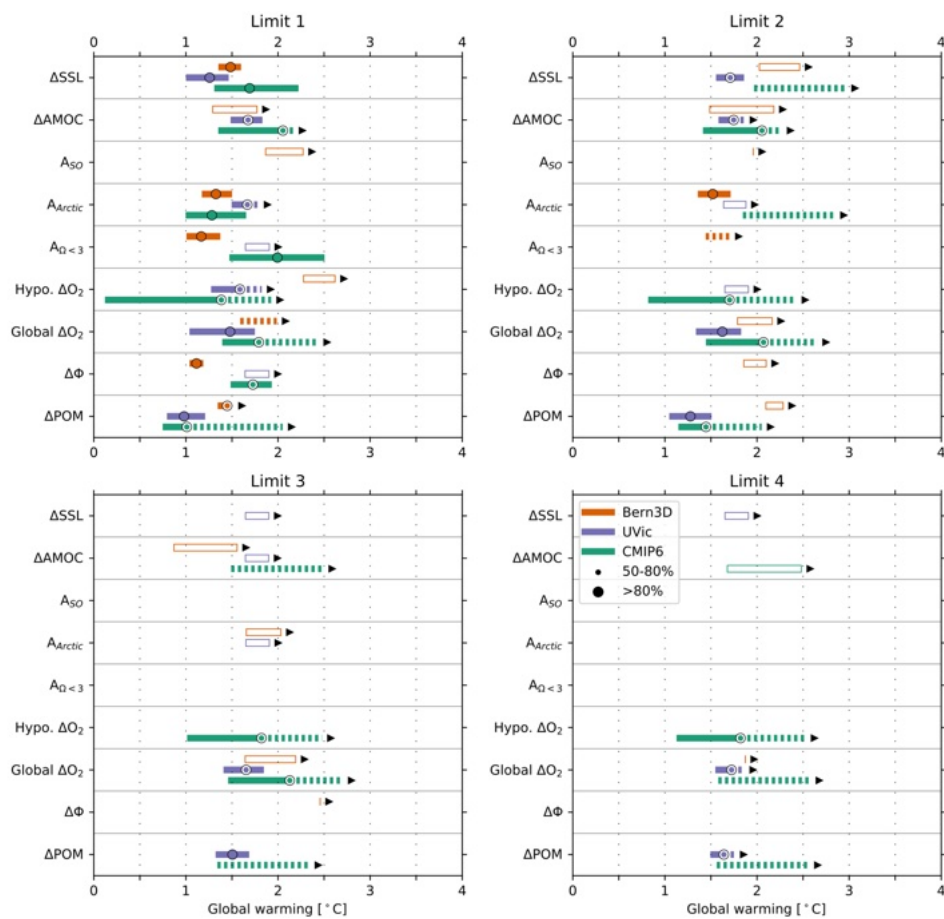
Figure A3: Same as in Figure 8 but for SSP1-2.6.
