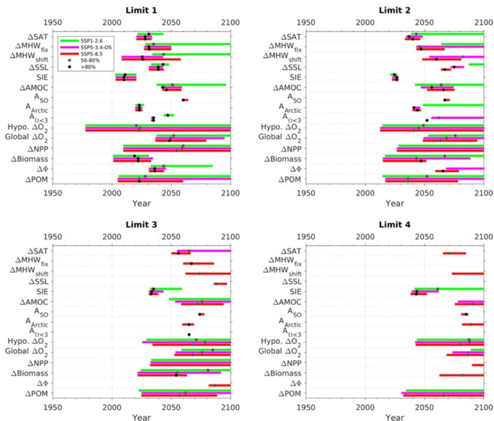
Figure 1: Box plots showing the distribution of exceedance years for each mitigation limits of the impact metrics (abbreviations follow Table 1) for CMIP6 models. Green, purple and red colors depict the three scenarios, i.e., historical-SSP1-2.6, historical-SSP5-3.4-OS and historical-SSP5-8.5. Boxes' lengths and circled black dots depict the interquartile range and the ensemble median, respectively. The size of the black dots indicates the exceedance probability defined as the proportion of models exceeding a mitigation limit across the models providing data for a given impact metric (Full size: >80 %, half size: 50-80 %). The median of low probability exceedances (<50% of models) are not shown.
