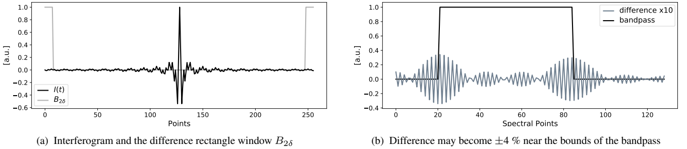
Figure 2. Simulation example where the shortening operation is applied to a double sided interferogram shown in (a) that corresponds to an idealized bandpass model shown in (b) (only positive frequencies are shown in the spectral domain, interferogram size N = 2^8 , bandpass width L = N/4 ). The effect in the spectral domain of removing \delta = 2^3 points at each end of the interferogram is shown. No apodization is used.
