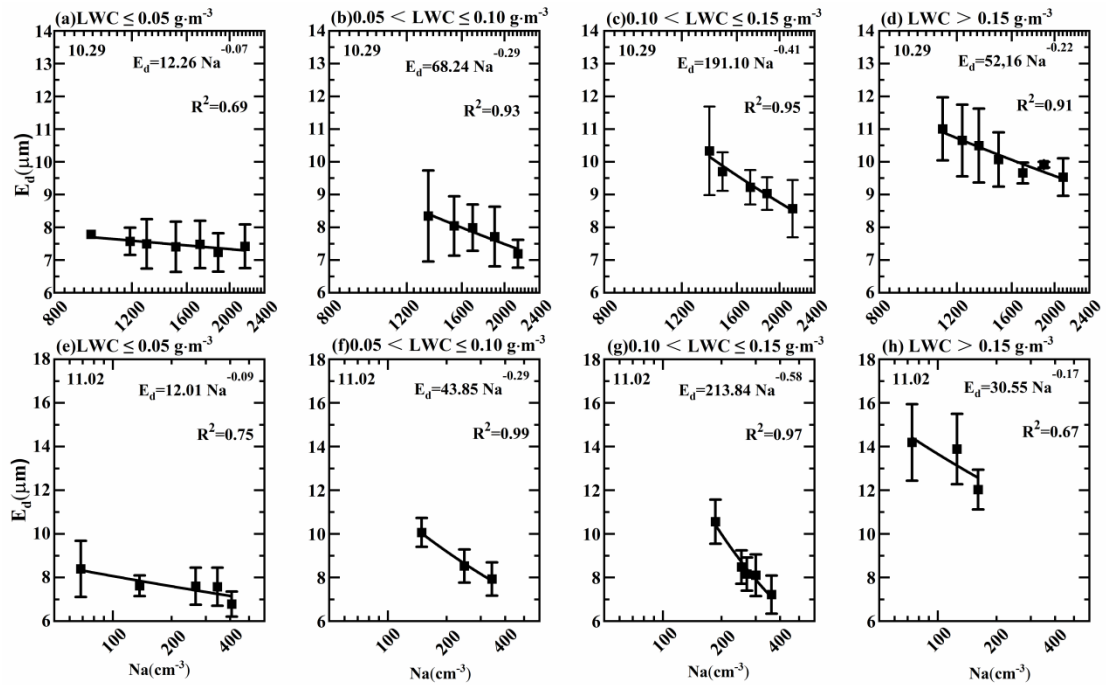
Fig. 10 Correlation between aerosol number concentration and effective droplet diameter in the range of 0-0.05, 0.05-0.10, 0.10-0.15 and > 0.15 \text{ g}\cdot\text{m}^{-3} LWC (a-d are October 29, e-f are November 2, R^2 is the correlation coefficient. The significance level \alpha was set at 0.05, and the P-value < 0.05 was obtained.)
