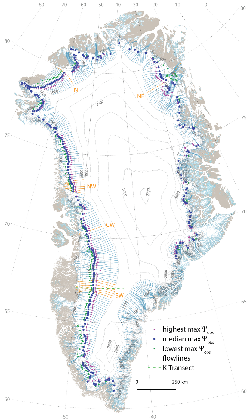
Figure 1. Median, highest and lowest of all annual MODIS \max \Psi_{obs} for the time period 2000 to 2021. Retrievals at the east coast between 60° to 68.4°N, where the hydrological regime is dominated by firn aquifers, have been masked. Flowlines highlighted in orange indicate the locations for which detailed results are shown in Figs. 2, 4, C1 and C2. The location of the K-transect (Figs. 5, 6 and C3) is indicated as well.
